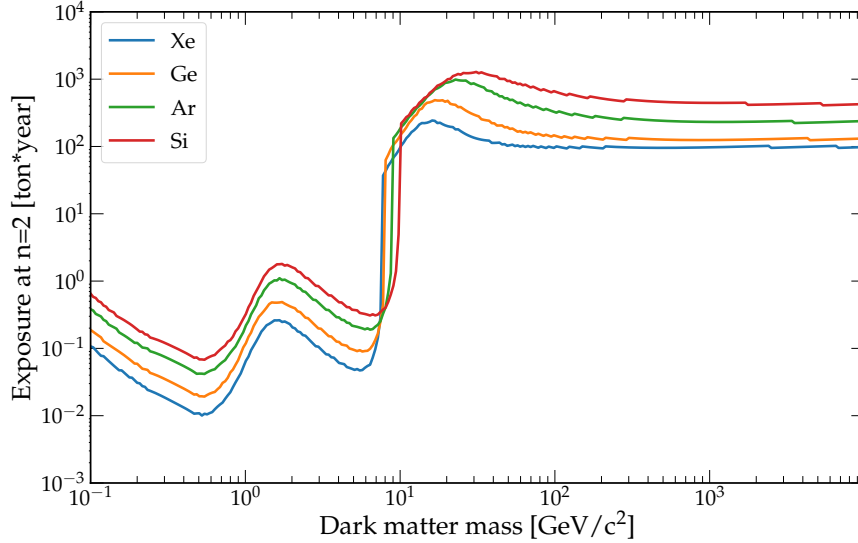
Figure 3: Exposure in ton-years required to reach the n = 2 (systematic-limited) spin-independent neutrino fog level as a function of dark matter mass for various targets.
