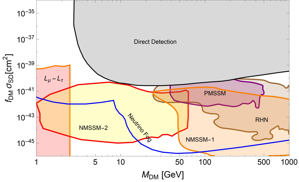
Figure 7: Plots of dark matter-proton cross section \sigma_{SD} times dark matter fraction f_{DM} versus particle mass M_{DM} for SD scattering cross sections off nuclei. Examples of predicted regions in several visible sector models are reproduced: the NMSSM models of [29] (“NMSSM-1”, in orange) and of [30] (“NMSSM-2”, in yellow), the pMSSM model of [35] (“pMSSM”, in purple), the U(1)_{L_\mu-L_\tau} gauge SM extension model of [40] (“ L_\mu - L_\tau ”, in pink), the heavy Dirac fermion model in [41] (“RHN”, in brown). The gray region is excluded by existing direct detection limits and the blue line indicates the neutrino fog level in for C_3F_8 [26].
