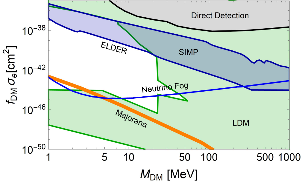
Figure 8: Dark matter-electron scattering cross section \sigma_e times dark matter fraction f_{\text{DM}} versus particle mass M_{\text{DM}} . Examples of predicted regions in several models are reproduced: the f_{\text{DM}} = 1 line for the ELDER model and region for the SIMP model of [51] (in blue), the Majorana dark matter line of Fig 6 of [24] (in orange), the symmetric and asymmetric light dark matter (LDM) region of [49] (in green). The 100% discrimination F_{\text{DM}} = 1 neutrino fog level for a 10^5 kg-y exposure of [28] (blue line) and the region rejected by present direct detection constraints (in grey) are shown for comparison.
