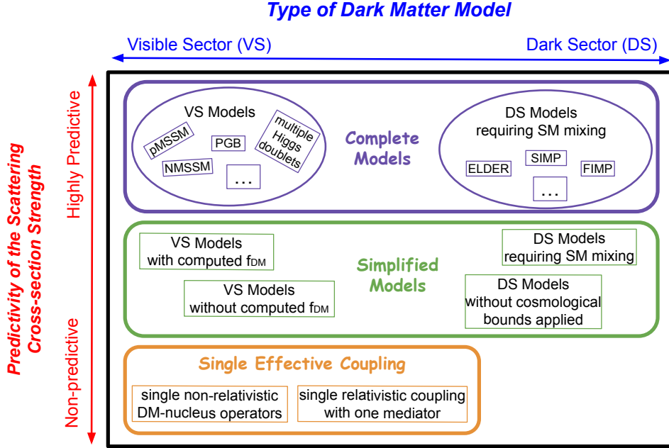
Figure 4: Landscape of models classified in terms of predictivity of scattering cross sections strength with nuclei or electrons (vertical axis) and from mostly built within the visible sector or a dark sector (horizontal axis), as explained in the text. Complete models are highly predictive, single effective coupling models are non-predictive, and simplified models are somewhere in between, in terms of predictivity. Examples of models that predict cross sections at the neutrino fog level are given in the text (FIMP or feebly interacting massive particles models typically predict cross sections much below the neutrino fog level in the dark matter mass range of interest here).
