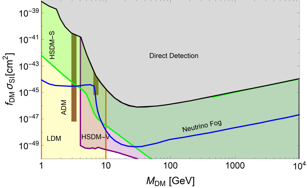
Figure 6: Same as in Fig. 5 for SI cross sections but for a few dark sector models: the minimal hidden sector dark matter models of [34] with a vector portal (“HSDM-V”, in purple) and with a Higgs scalar portal (“HSDM-S”, in green), the asymmetric dark matter model of [48] (“ADM”, brown vertical bars) and the symmetric and asymmetric light dark matter models of [49] (“LDM”, in yellow).
