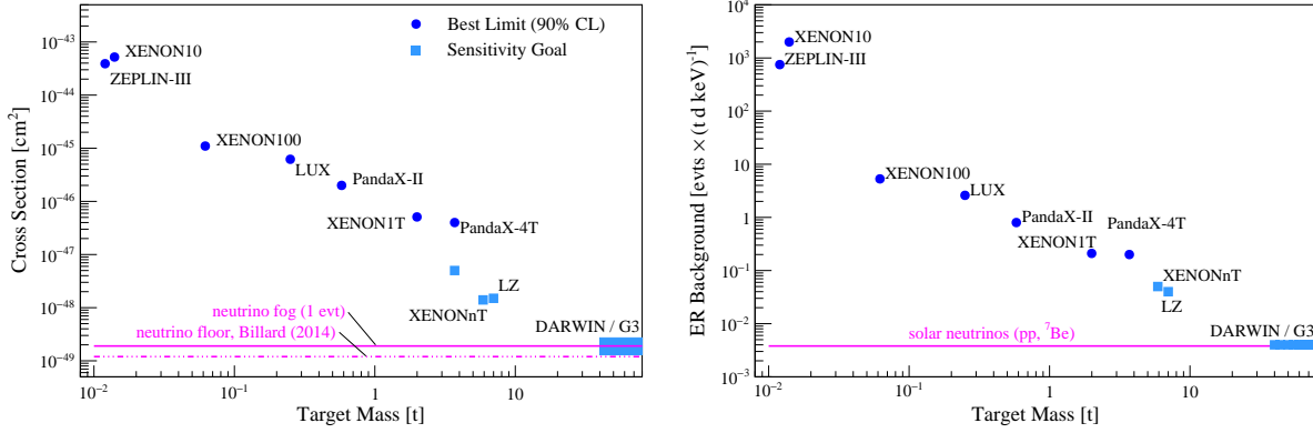
Figure 9: (left) Development of LXe-TPC technology. The plot shows the improvement in sensitivity to spin independent WIMP-nucleon coupling (for a mass of 50 \text{ GeV}/c^2 ) achieved by LXe experiments of increasing target masses. Sensitivity goals are also reported for experiments that have not yet been completed. (right) The plot shows, as function of the target mass, the progress made in terms of background suppression. Cross section values and background rates are extracted from Ref. [68, 69, 72–79].
