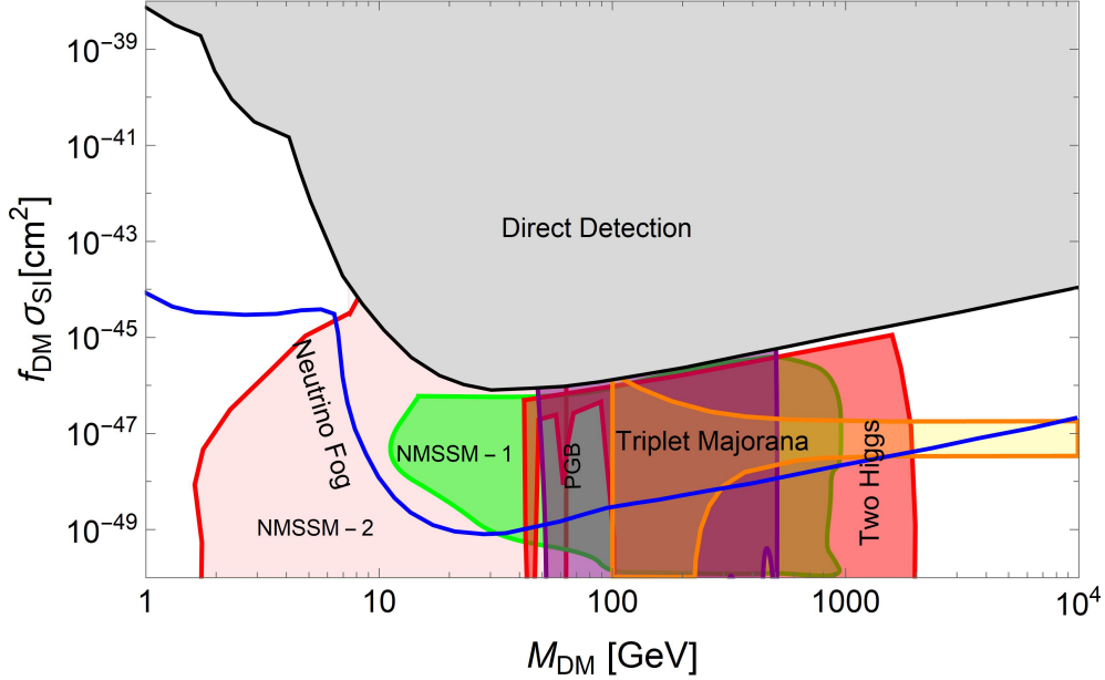
Figure 5: Plots of dark matter-proton cross section \sigma_{\text{SI}} times dark matter fraction f_{\text{DM}} versus particle mass M_{\text{DM}} for SI scattering cross sections off nuclei. Examples of predicted regions in several visible sector models are reproduced: the NMSSM models of [29] (“NMSSM-1”, in green) and of [30] (“NMSSM-2”, in pink), the two Higgs doublet model of [31] (“Two Higgs”, in red), the pseudo-Goldstone boson of [32] (“PGB”, in purple) and the electroweak triplet Majorana dark matter model of [33] (“Triplet Majorana”, in yellow - however note that the relic abundance for this model was not computed). The gray region is excluded by existing direct detection limits [34] and the blue line indicates the neutrino fog level in xenon [20, 26]. Regions predicted by other examples of models mentioned in the text [33, 35–39] overlap with those shown and were not included for clarity.
