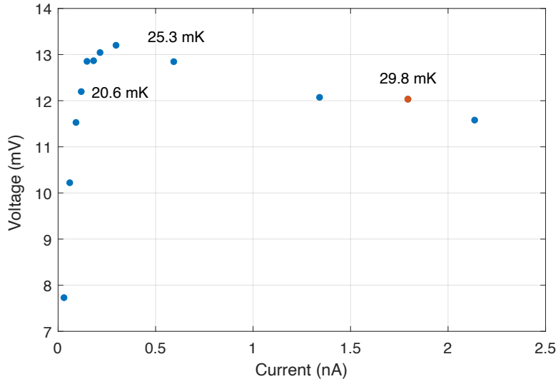
Figure 3. The IV curve of LD9 at a floating plate temperature of 15 mK. The plot shows also the temperature of the NTD at difference biases. The red dot represents the optimum working point (the best S/N ratio) that corresponds to an NTD resistance of 6.7 \text{ M}\Omega (29.8 mK temperature).
