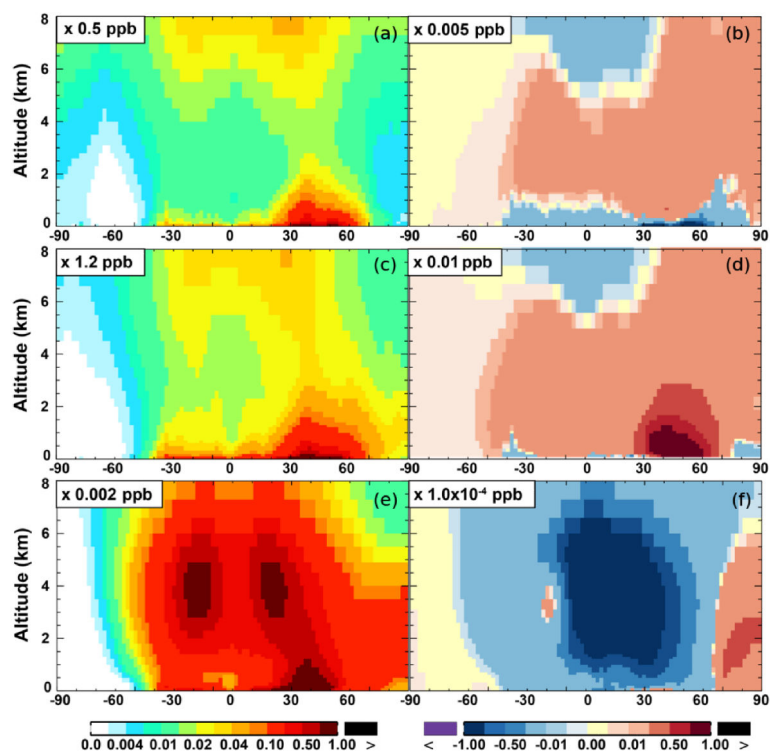
Figure 7. (a, c, e) Modeled zonal average latitude-altitude distributions of annual mean NO (a, b) and NO 2 (c, d) , and NO 3 (e, f) simulated in the Base scenario for the year 2005. (b, d, f) The respective changes from Base to SAPRC.
