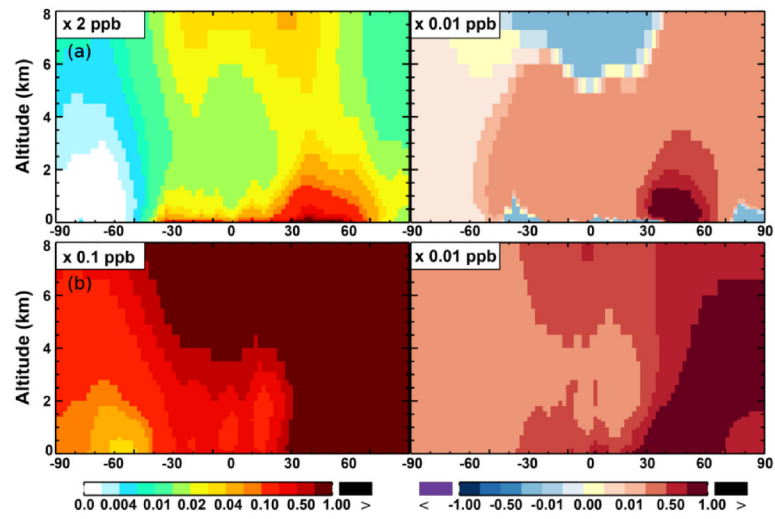
Figure 9. Same as Fig. 7 but for NO x (a) and PAN (b).
