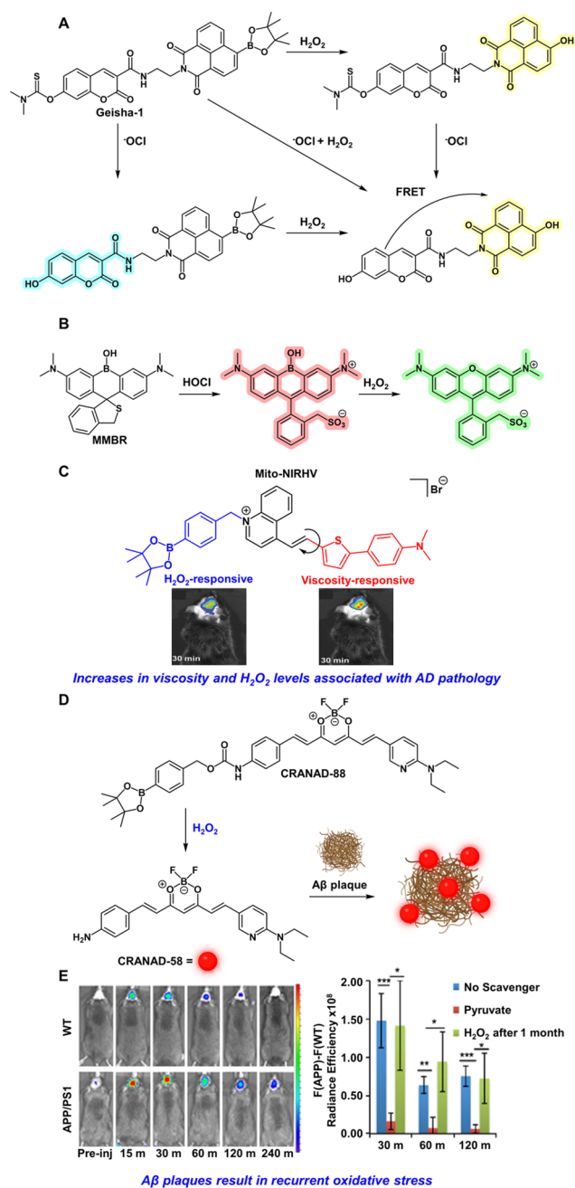
Figure 5. (A) Scheme depicting HOCl and \text{H}_2\text{O}_2 dual-sensing of Geisha-1. (B) Scheme depicting sequential HOCl and \text{H}_2\text{O}_2 mediated sensing by MMBR. (C) Mito-NIRHV simultaneously measures \text{H}_2\text{O}_2 and changes in viscosity and has been applied to in vivo mouse models of AD pathology. Adapted with permission from ref 101. Copyright 2020 The Royal Society of Chemistry. (D) CRANAD-88 responds to \text{H}_2\text{O}_2 to generate fluorescent CRANAD-58 which upon binding to \text{A}\beta plaques undergoes fluorescence amplification. (E) CRANAD-88 was applied to monitor both \text{H}_2\text{O}_2 and plaque formation in in vivo AD mouse models. Adapted with permission under a Creative Commons CC BY license from ref 100. Copyright 2016 Springer Nature.
