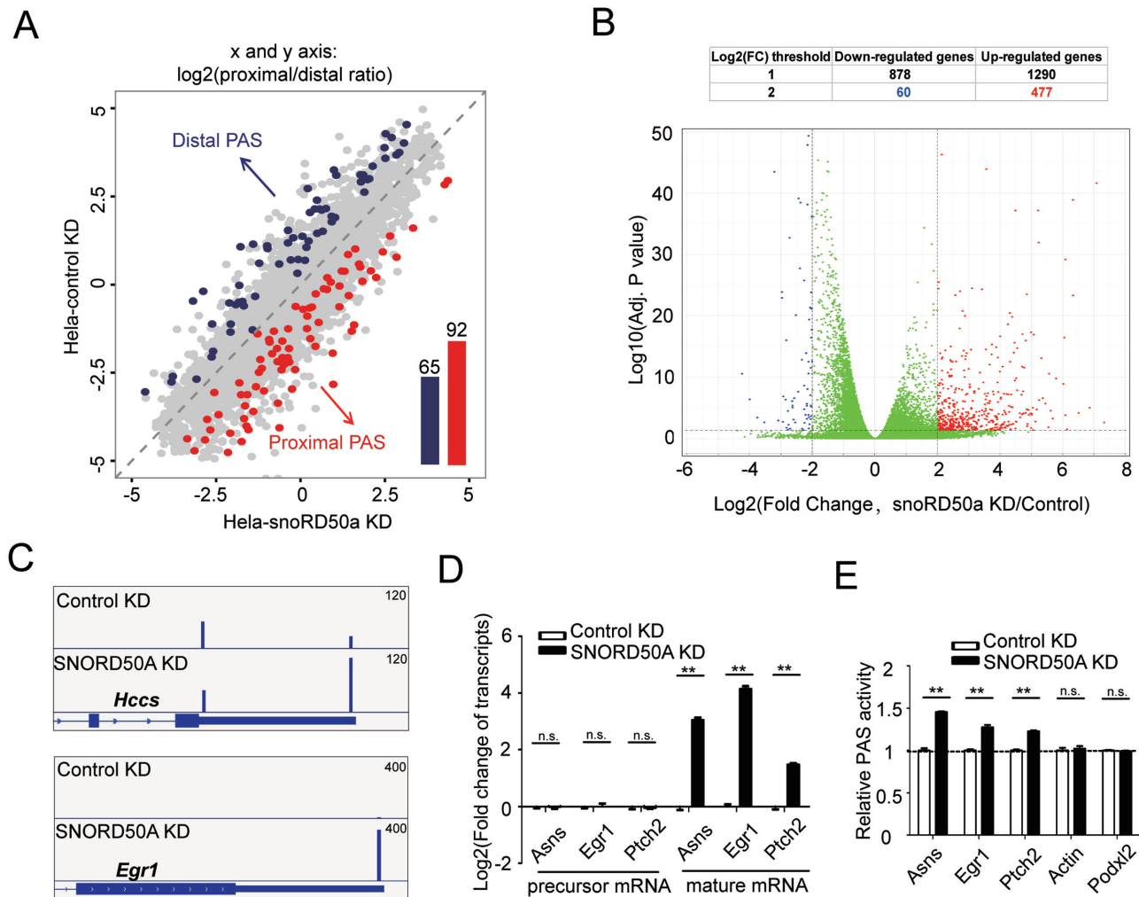
Figure 3. Effect of SNORD50A depletion on the 3' processing and expression level of endogenous poly(A) + transcripts. (A) PAS-seq analysis of APA in HeLa cells 2 days after they were transfected with NC ASO or SNORD50A ASO (ASO-1 and ASO-2 as a group), Log 2 (proximal/distal ratio) are plotted for HeLa cells transfected with NC ASO (y-axis) and SNORD50A KD ASO (x-axis). Statistically significant changes are highlighted in blue (proximal to distal shift) and red (distal to proximal shift). The numbers of APA changes are shown in the column graph. (B) Volcano plot showing the expression level change of poly(A) + mRNA in HeLa cells 2 days after they were transfected with NC ASO or SNORD50A ASO (ASO-1 and ASO-2 as a group). Highly reliable changes ( P < 0.05 , fold change > 4 ) were colored with red (up-regulated in SNORD50A KD cells in comparison to NC KD cells) or blue (down-regulated in SNORD50A KD sample in comparison to NC KD cells), green dots shows the changes either not statistically significant ( P > 0.05 ) or less reliable (fold change < 4 ). (C) IGV tracks showing the PAS-seq results for Hccs , Egr1 genes in HeLa cells with NC (top) or SNORD50A KD (bottom). (D) RT-qPCR analysis monitoring the relative expression levels of 3 mature and precursor transcripts in HeLa cells 2 days after they were transfected with NC ASO or SNORD50A ASO. Fold changes are relative to Gapdh and normalized to NC ASO control, plotted as mean \pm S.E.M. ( n = 3 ). Student's t-test was used to determine the significance of the change. n.s.: not significant; ** P < 0.01 . (E) Luciferase reporter assays are similar to Figure 2D except that the targets are 5 endogenous mRNAs PASes instead of SVL PAS. Student's t-test was used to determine the significance of the PAS activity change, ** P < 0.01 .
