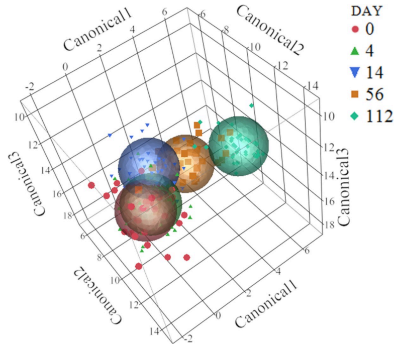
Fig 5. Linear discriminant analysis of the 28 microbial functions from Level 1. Changes in microbial genetic function over time ( P -value < 0.05). An ellipse indicates the 95% confidence region to contain the true mean of the variable (day).
