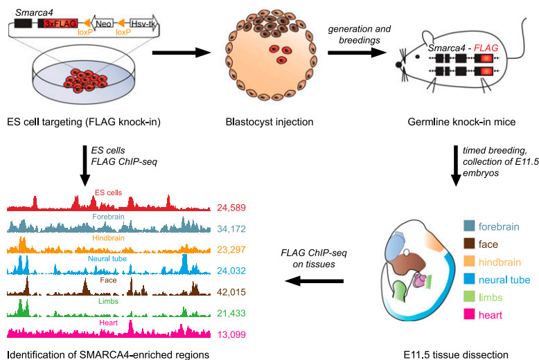
Figure 1. Overview of Smarca4 FLAG mouse generation and SMARCA4 binding site mapping in vivo. A knock-in mouse strain carrying a FLAG epitope at the carboxy terminus of SMARCA4 was engineered and used to perform ChIP-seq from a panel of embryonic tissues. For each ChIP-seq data set, the total number of identified enriched SMARCA4 regions is indicated near the corresponding coverage map (schematics).
