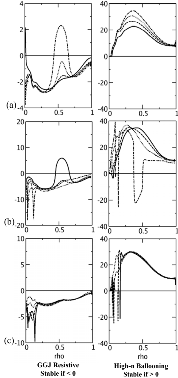
Fig. 3. GGJ resistive and high- n ideal ballooning criteria of profiles A (solid lines), B (dashed lines), C (dash-dot lines) and D (dotted lines) for (a) peak location, (b) peaking factor and (c) transition scans. The different criteria are plotted as a function of \rho ( =r/a ). \rho = 0 is at the magnetic axis and \rho = 1 at the plasma edge. The ordinates of all curves are in arbitrary absolute units. In the left column, the part of the profiles that is positive shows instabilities to resistive interchange instabilities. In the right column, the profiles are stable is the criterion is positive.
