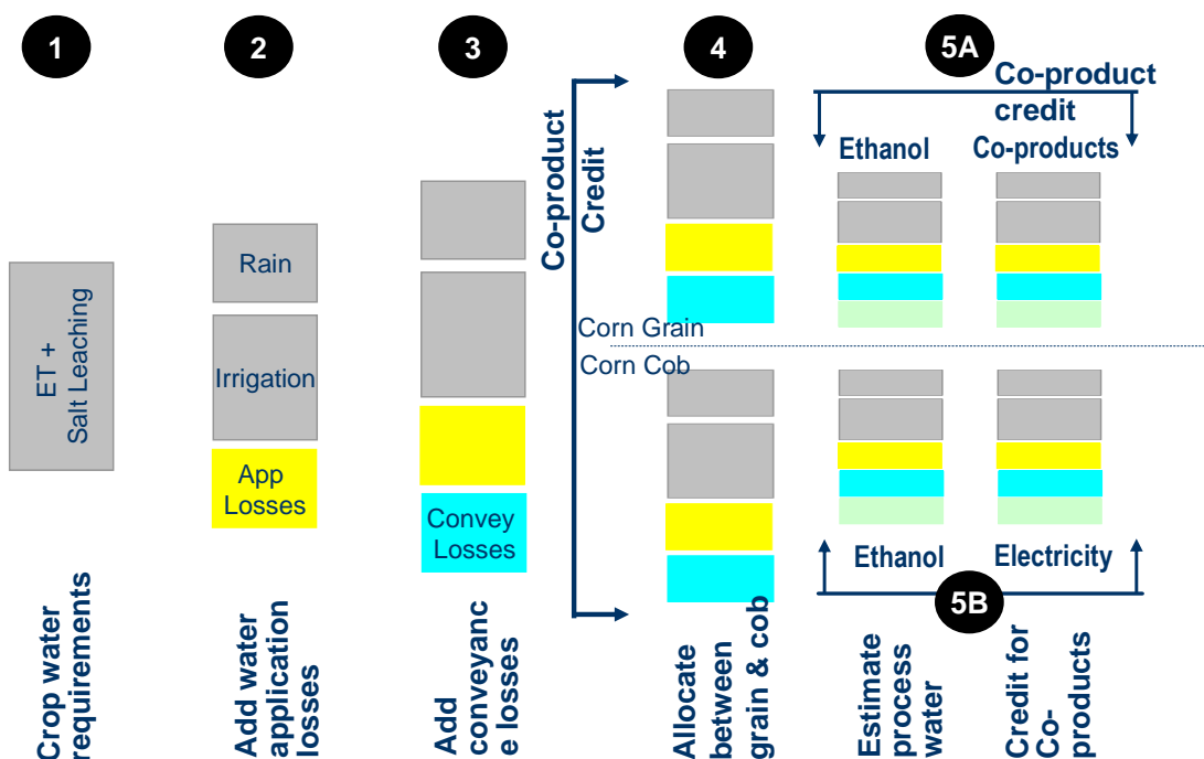
Figure 3.1: Framework for estimation of water requirements of ethanol from corn and crop residue (corn cob)
