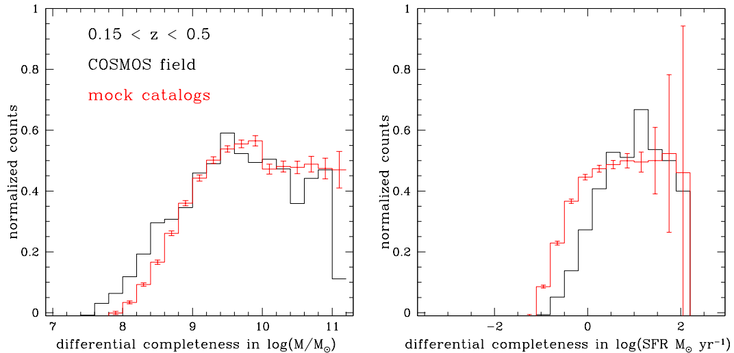
Figure 3. Left panel: spectroscopic completeness per stellar mass bin in the low redshift sample (black histogram) and in the simulated “incomplete” mock catalog (red line) in the same redshift range. Right panel: spectroscopic completeness per SFR bin for the low redshift sample (black histogram) and in the simulated “incomplete” mock catalog (red line).
