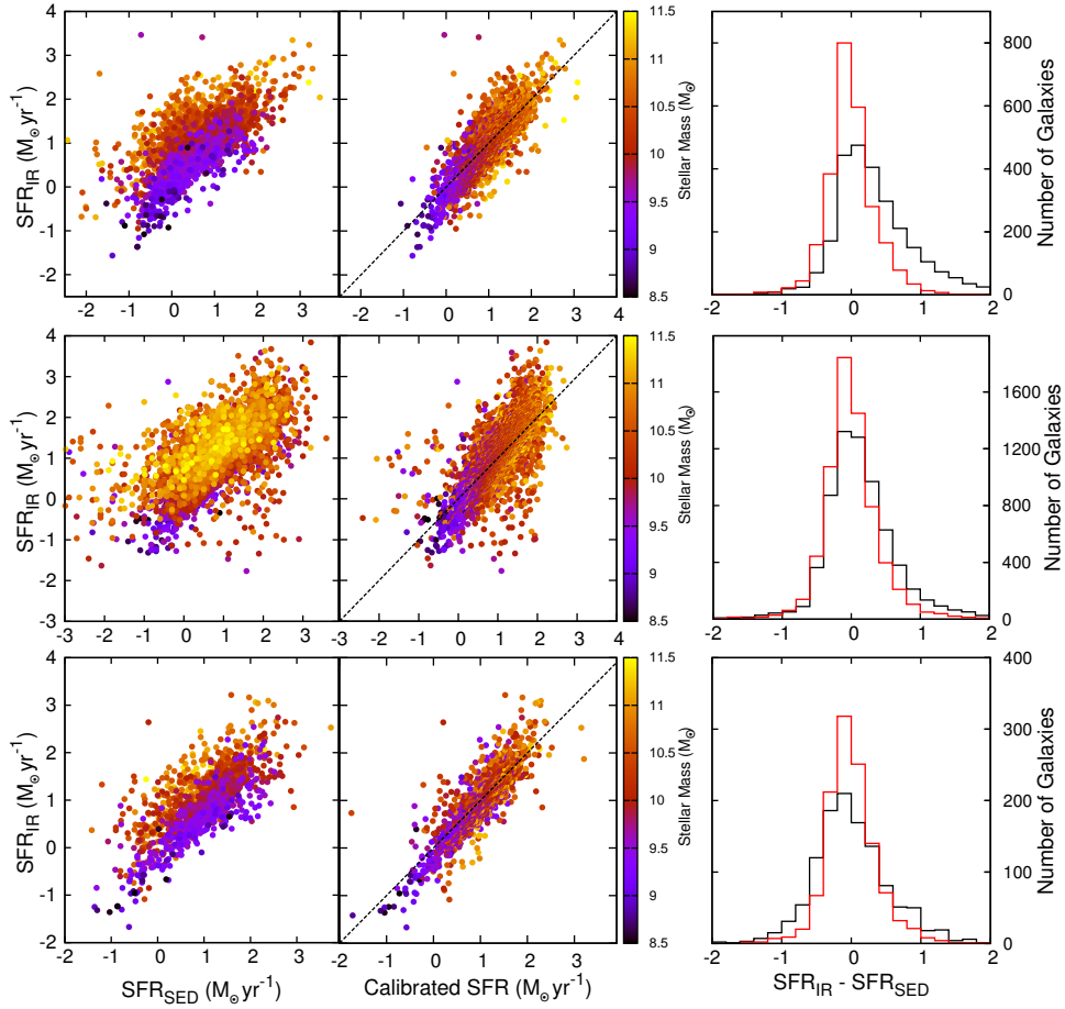
Figure 2. The left panels show SFR_{IR} vs. SFR_{SED} color-coded by stellar mass before re-calibration for EGS, COSMOS and GOODS-S from top to bottom respectively. The middle panels show corresponding SFR_{IR} vs. re-calibrated SFR_{SED} . The dashed line is one to one relation. The right panels are the histogram of corresponding SFR_{IR} - SFR_{SED} . The black and red histograms show before (black) and after (red) re-calibration.
