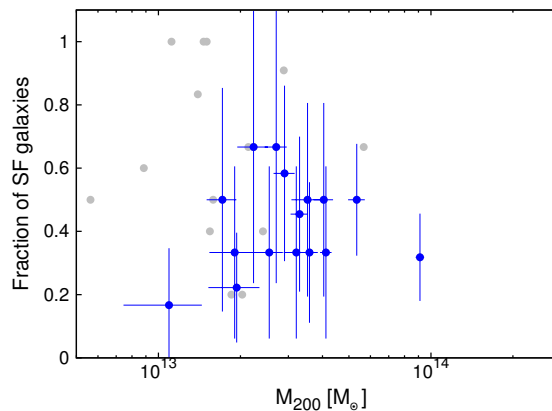
Figure 14. Fraction of star-forming galaxies as a function of halo mass for the low- z sample with more than 10 members (blue points) and less than 10 members (in grey). Spearman test confirms no correlation for this sample.
