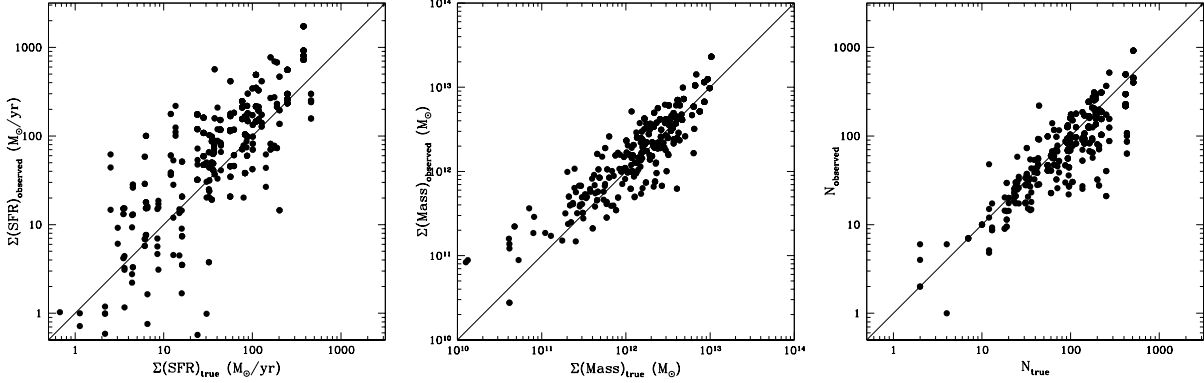
Figure 9. From left to right, “True” values of total SFR, total stellar masses and halo occupation number of the groups vs. our estimates in the “incomplete catalogs” with the same level of spectroscopic incompleteness of the surveys used in this work.
