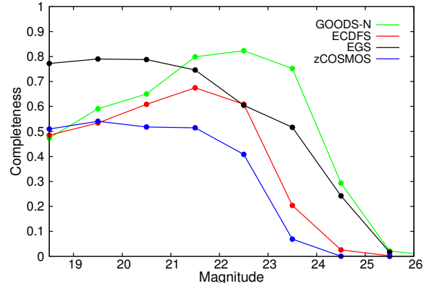
Figure 5. Spectroscopic completeness for different fields in R-band magnitude. We use v -band magnitude for GOODS-N.
