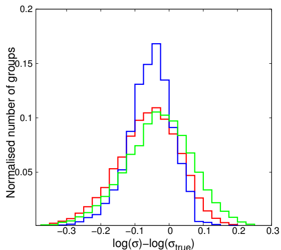
Figure 7. Distribution of the residuals of the logarithm of the “true” and “observed” velocity dispersion. The blue histogram shows the distribution of the residuals obtained from the original mock catalogs. The red histogram shows the distribution obtained if we take into account the error on M_{200} derived from L_X as done in the real dataset. The green histogram shows the same diagram but with the “observed” velocity dispersion estimated on the basis of the “incomplete” mock catalog.
