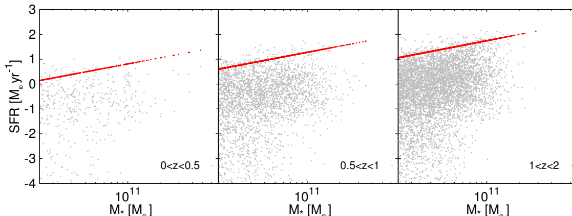
Figure 18. SFR as a function of stellar mass for the member galaxies in the mock catalog. The red points show the position of the main sequence for the lowest redshift ( z = 0, 0.5 and 1 from left to right, respectively) in each bin.
