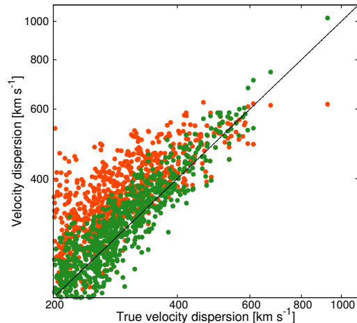
Figure 8. Velocity dispersion from gapper estimator vs. true velocity dispersion for mock groups. The orange points show the choice of constant initial velocity dispersion and the green one is based on the initial velocity dispersion computed from M_{200}
