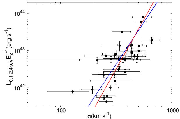
Figure 1. L_X - \sigma relation for X-ray groups. The dashed blue line show our expectation for L_X - \sigma relation from scaling relations (Leauthaud et al. 2010) and the solid red line is our bisector fit to data.
