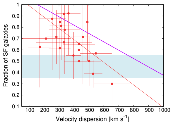
Figure 16. Fraction of star-forming galaxies vs. velocity dispersion for groups in the high- z sample with more than 10 spectroscopic members. The magenta line is the upper envelope of Poggianti et al. (2006) for the EDisCS clusters and groups at z=0.4-0.8 . The horizontal blue line and the shaded blue area show the median fraction of star-forming galaxies and its corresponding one sigma error in low- z groups.
