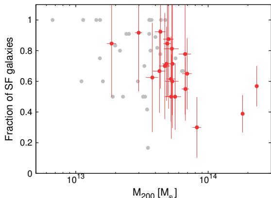
Figure 15. Fraction of star-forming galaxies as a function of halo mass for the high- z sample with more than 10 members (red points) and less than 10 members (in grey). Spearman test confirms a significant anticorrelation for the this sample.
