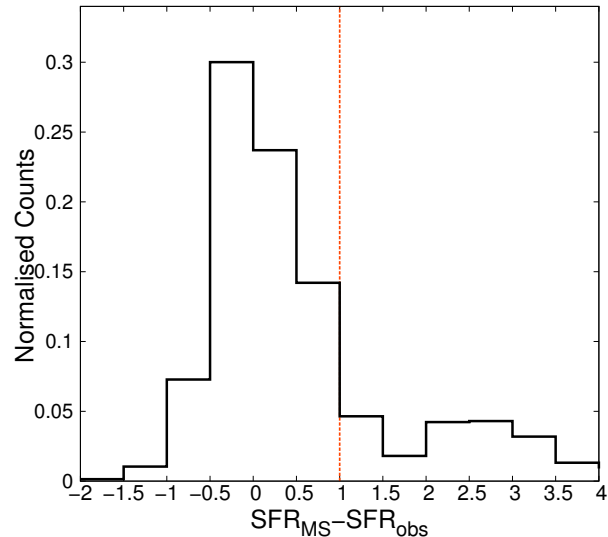
Figure 13. Normalized distribution of differences between Main Sequence SFR and observed SFR of member galaxies ( \Delta\text{SFR} ). The red vertical lines show our limit for separation MS member galaxies.
