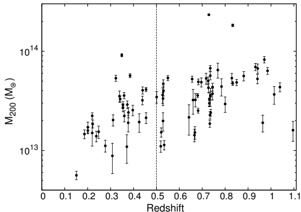
Figure 4. M_{200} vs. redshift for the final sample of galaxy groups in our analysis. The vertical dashed line separates low- z and high- z sample.
