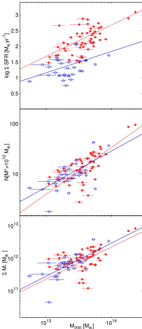
Figure 10. \Sigma SFR- (upper panel), N- (middle panel) and \Sigma M_* - (bottom panel) M_{200} relations for member galaxies with M_* > 10^{10} M_\odot in the low- z sample ( 0.15 < z < 0.5 , in blue) and the high- z groups ( 0.5 < z < 1.1 , in red). The blue and red lines show the best-fitting using the ordinary least squares regression method presented by Akritas & Bershady (1996). The total star formation activity in high- z groups is higher with respect to the low- z sample at any mass by 0.8 \pm 0.12 dex. The N- and \Sigma M_* - M_{200} are consistent with a linear relation in both redshift bins with no evolution since z \sim 1.1 .
