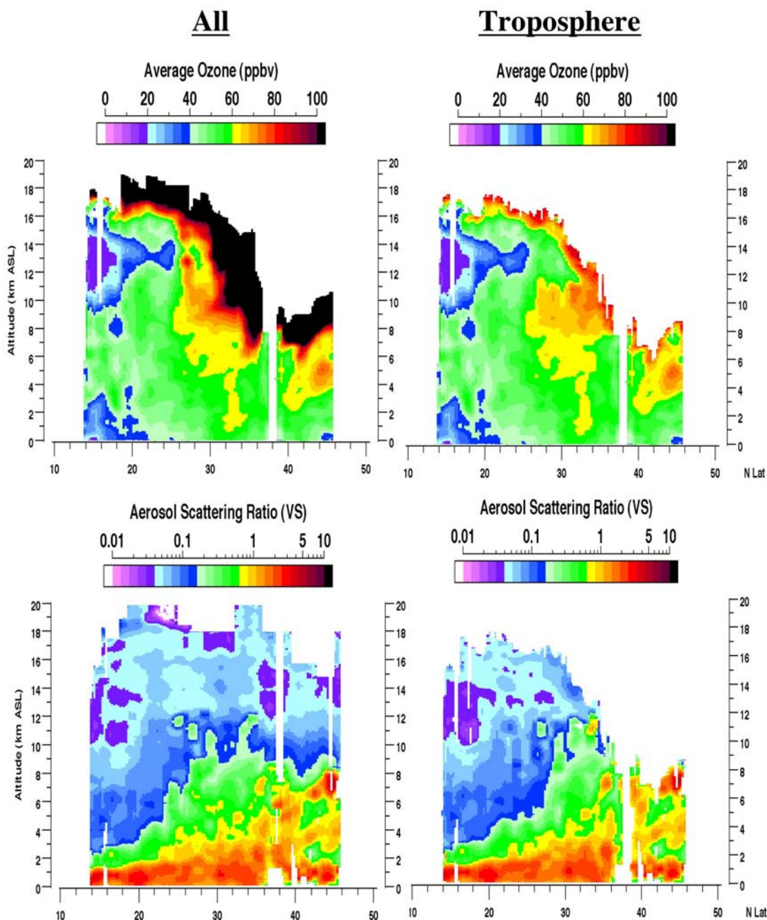
Figure 4. Average latitudinal \text{O}_3 (top) and aerosol (bottom) distributions observed during TRACE-P over the western Pacific (west of 150^\circ\text{E} ). Left panels include all data (tropospheric and stratospheric) and right panels include only tropospheric data.
