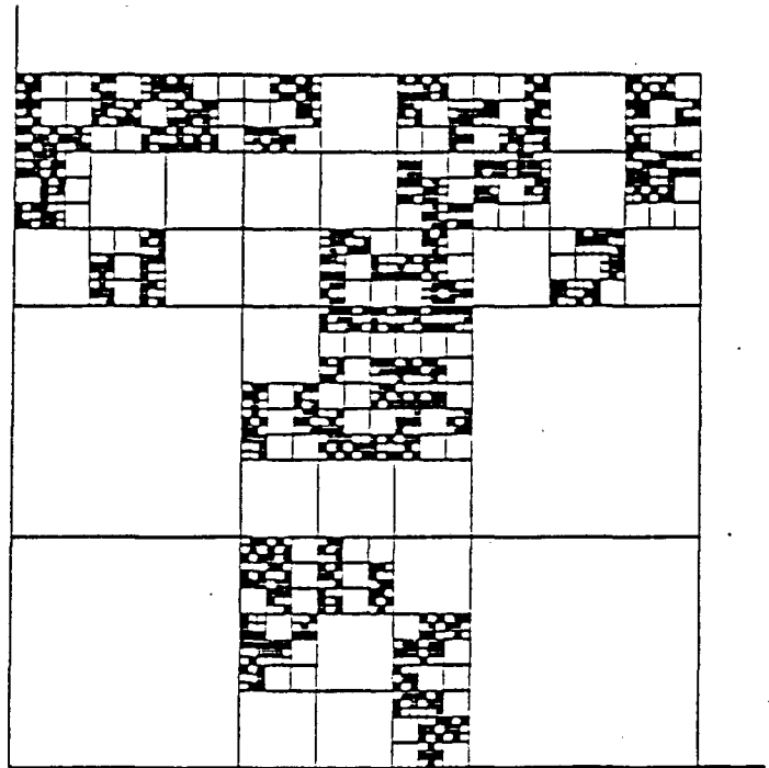
Figure 13. Well test results in a fractal network.
