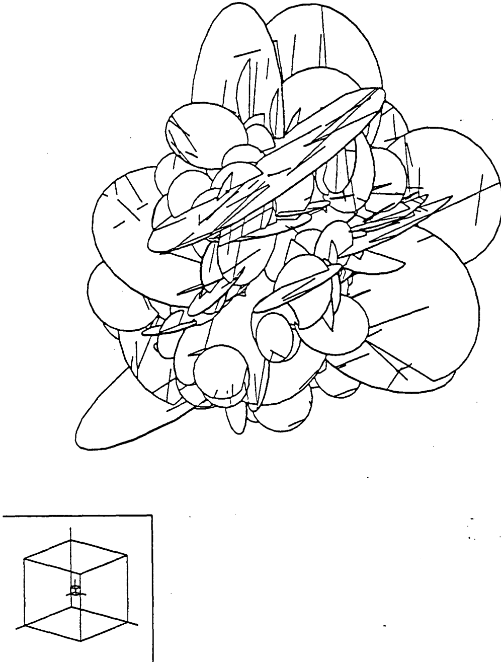
Figure 1. Shown are the 220 fractures with diameters larger than 1m intersecting a sphere with a 2.5m radius based on data from the Fanay- Augres.
