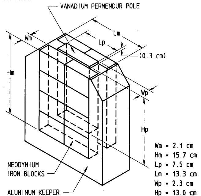
Figure 1. Half Period Pole Assembly
