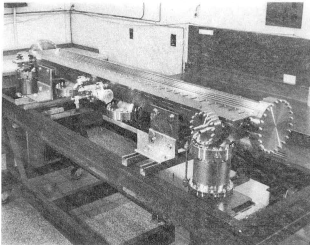
Figure 5. BLX Wiggler Vacuum Chamber
