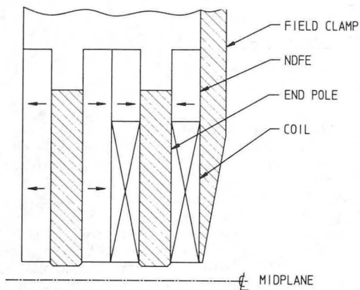
Figure 2. End Pole Configuration
