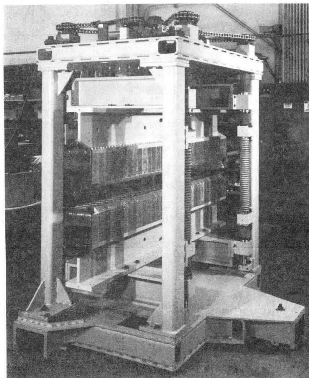
Figure 4. Beam Line X Wiggler
