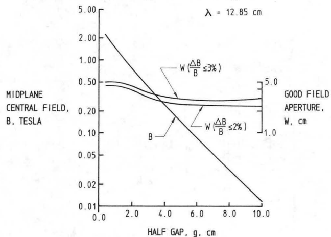
Figure 3. Prototype Pole Magnetic Measurements
