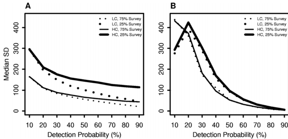
Figure 3. Median standard deviation of population estimates. The figures show the changes in median standard deviation (SD) relative to detection probability for the low (LC) and high clustered (HC) populations at survey proportions of 25% and 75% for the double observer and double sampling methods (Panels A and B, respectively). Median standard deviation for the double observer method is larger than for the double sampling method at low detection probabilities but is very small at high detection probabilities. doi:10.1371/journal.pone.0003047.g003
