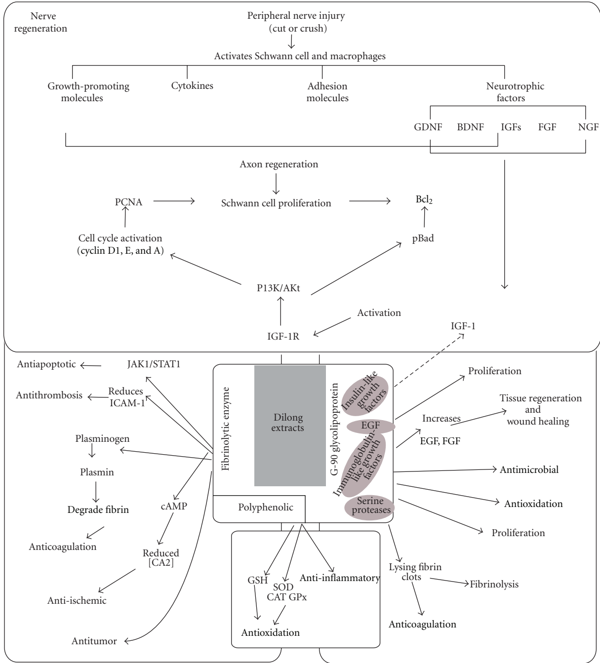
FIGURE 1: Schematic model of the survival and proliferative effects of Dilong extract on RSC96 Schwann cell. Stimulation of Schwann cell with Dilong extract activates IGF-I signaling, leading to upregulation of the PI3K/Akt pathway and activation of the cell cycle regulatory proteins cyclin D1, E, and A, resulting in the survival and proliferation of RSC96 Schwann cell. Dotted lines indicate the hypothetical molecular mechanism of the bioactive compound present in Dilong powder (from [40]).
