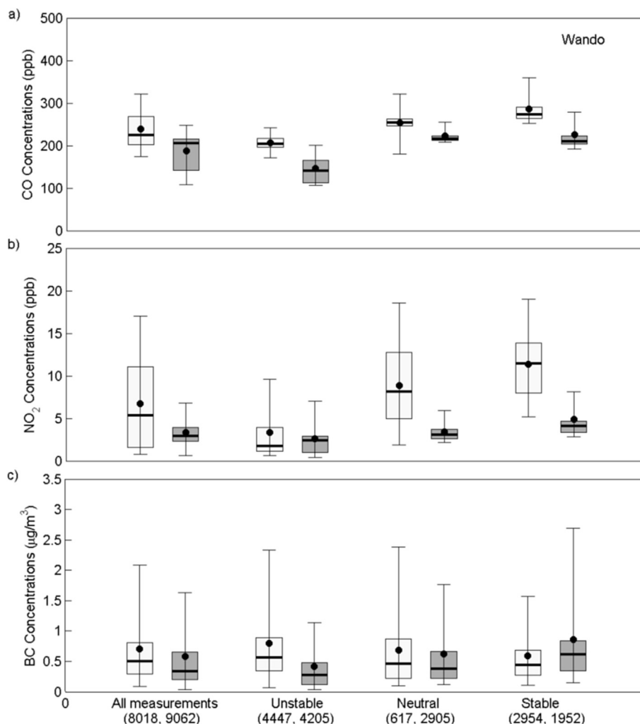
Fig. 9. Distributions of observed CO (a), \text{NO}_2 (b), and BC (c) concentrations from mobile monitoring downwind (light gray) and upwind (dark gray) of Wando Welch terminal for various stability conditions during the entire study. Each distribution is based on n observations (shown in parentheses below labels). The middle line represents the median, the box the 25th and 75th percentiles, and the whiskers the 5th and 95th percentiles. The data point represents the mean value of the distribution.
