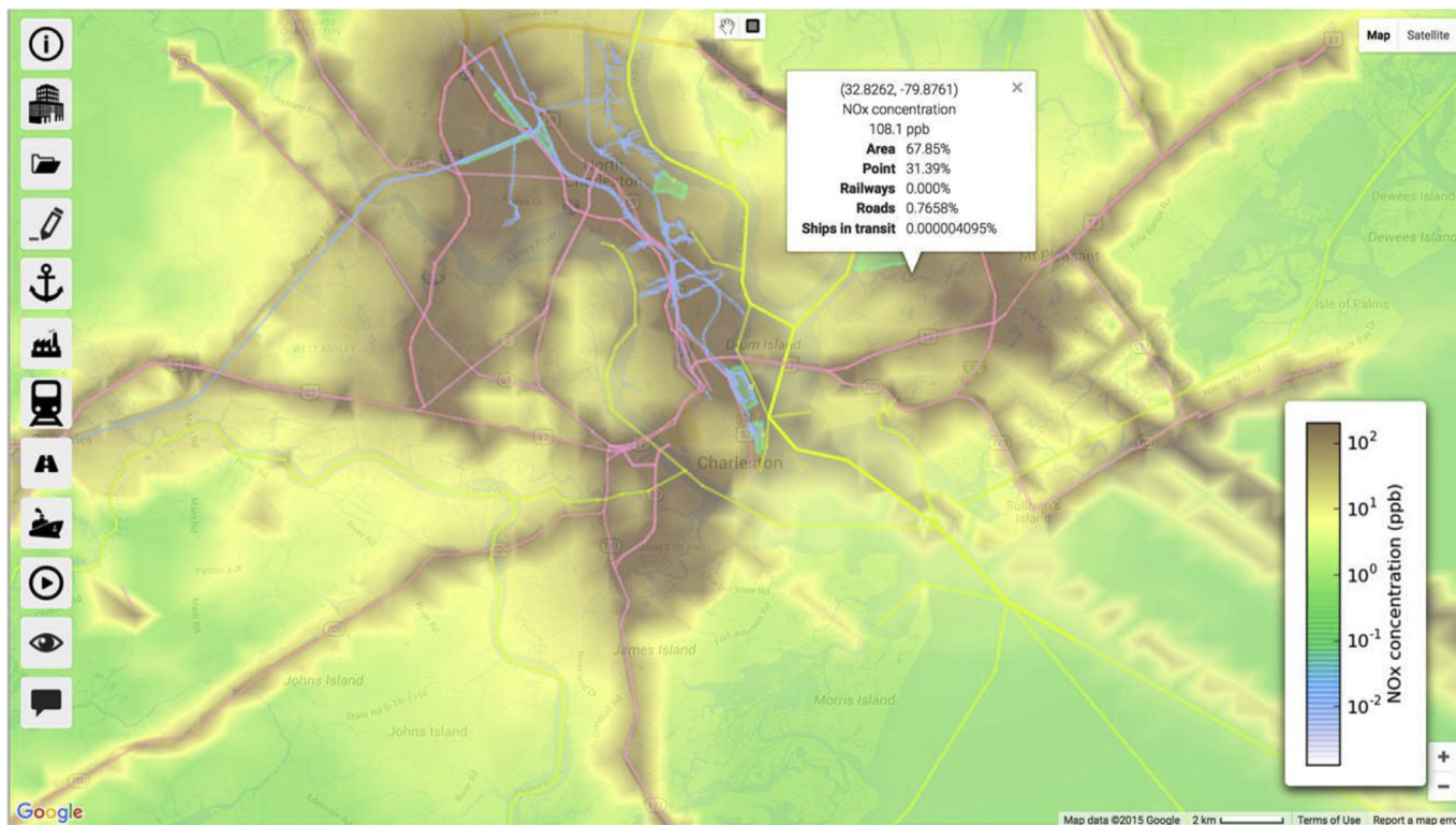
Fig. 7. Example of C-PORT application in Charleston, SC, showing NOx concentrations.
