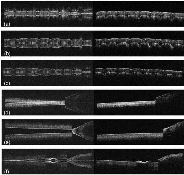
Fig. 4 In vivo images of human fingerpads and fingernails acquired at different image acquisition speeds with standard FD-OCT reconstruction (left column) and the full-range reconstruction with the sample arm pivot offset phase-shifting ( \Delta\varphi=0.5\pi ) method (right column). Human fingerpad at (a) 20-fps, (b) 50-fps, and (c) 100-fps B-scans. Human fingernail at (d) 20-fps, (e) 50-fps, and (f) 100-fps B-scans. The lateral scanning range is 6 mm.
