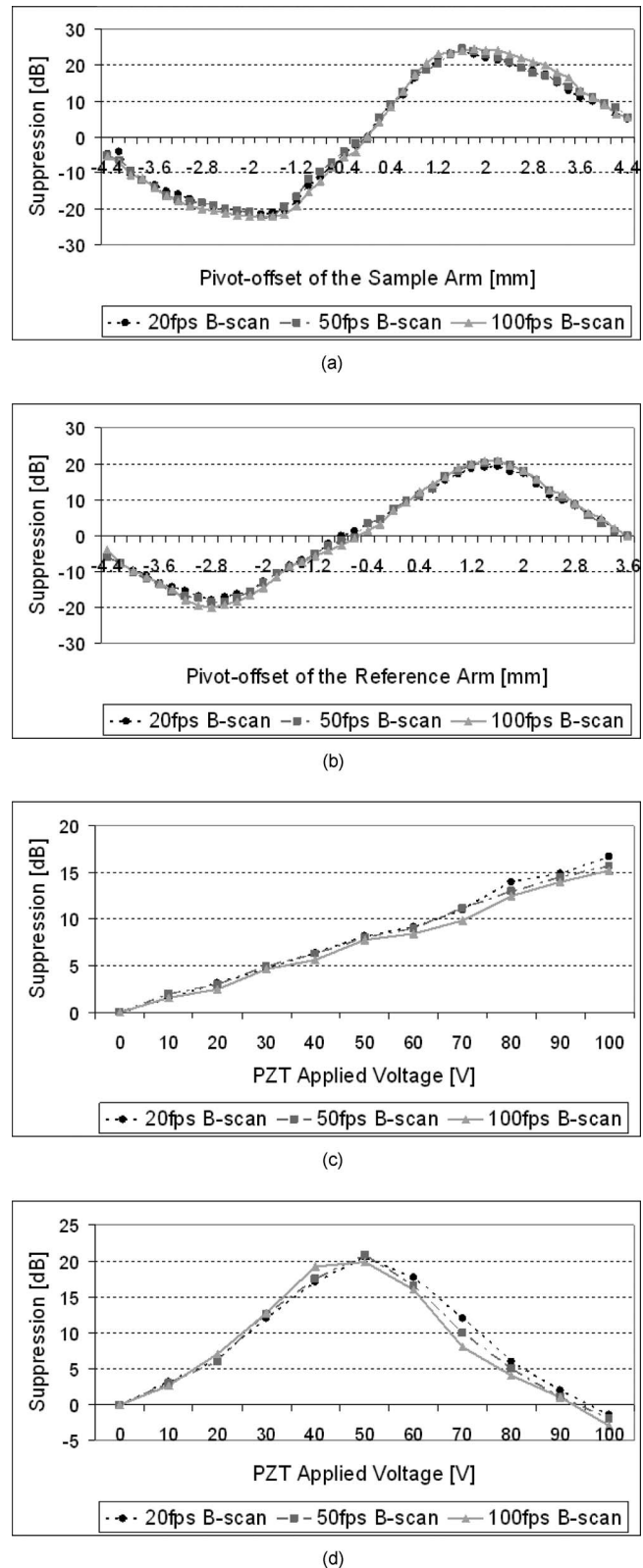
Fig. 3 Suppression ratio of complex conjugate artifacts using a paperboard with: (a) pivot offset scanning of the sample arm; (b) pivot offset scanning of the reference arm; (c) phase shifting with the PZT, 1000 A-scans, and 6-mm scanning range; and (d) phase shifting with the PZT, 300 A-scans, and 1.5-mm scanning range.
