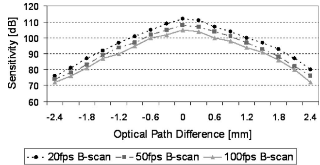
Fig. 2 System sensitivity measurement as a function of optical path length difference and different acquisition speeds.
