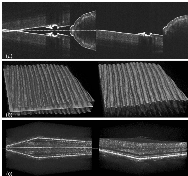
Fig. 7 In vivo standard FD-OCT images (left) and full-range images (right) after reconstruction of the complex-conjugate-free methods. (a) High resolution fingernail images at 100-fps B-scan without and with the sample arm pivot offset method ( \Delta\varphi=0.5\pi ). The lateral scan range of the images is 6 mm. (b) 3-D visualization of a human fingernail at 100-fps B-scan without and with the reference arm pivot offset method ( \Delta\varphi=0.5\pi ). The image size is 8.5(x) \times 8.5(y) mm. (c) In vivo 3-D human retinal imaging at 100-fps B-scan without and with the reference arm pivot offset method ( \Delta\varphi=0.5\pi ). The region of interest is 3(x) \times 3(y) mm. The dashed line is the zero path length difference position.
