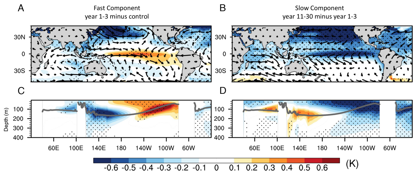
Fig. 3. The fast and slow responses in the idealized aerosol experiments. (A and B) Spatial patterns of SST (shaded) and surface wind stress (vector) anomalies. (C and D) Vertical structure of potential temperature anomalies along the equator (5°S–5°N mean) as a function of depth (m). Dotted region indicates statistically significant values of temperature anomalies at the 95% confidence level based on two-sided t test.
