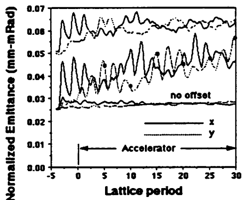
Fig. 7 Beam emittance variations in the x and y planes for offset beams drifted through MBE-4 obtained from code simulations.
