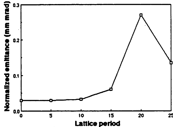
Fig. 10 Measurements of beam emittance along MBE-4 for the case of maximum current growth above.
