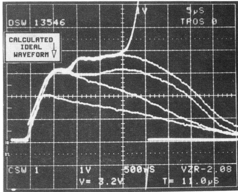
Fig. 3. Synthesis of MBE-4 accelerator wave forms. The outputs of four pulsers are added to produce an accelerating voltage close to that requested by the SLID acceleration procedure (XBB 872-1623)
