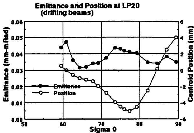
Fig. 6. Variations of beam position and emittance versus focus strength at lattice point 20. Varying focus strength brings the beam fluctuations to the point of diagnostic access.
