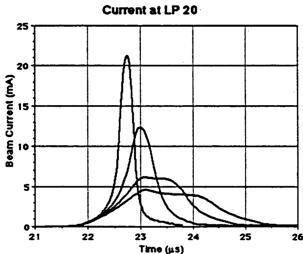
Fig. 9. Measurements of beam current at lattice point 20 for various beam tilts applied at the first four accelerating gaps. The lowest curve was obtained for no applied acceleration.
