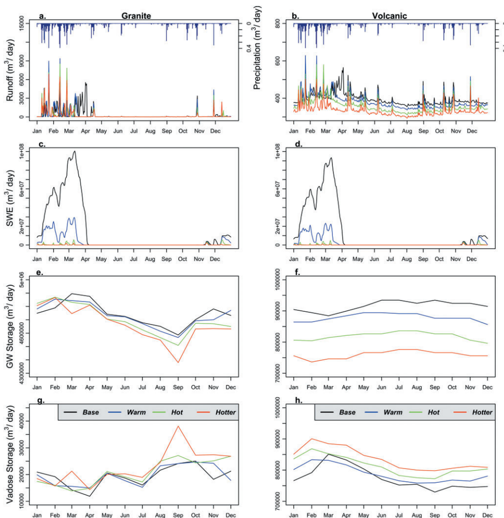
Figure 3. Summary figure of the storage values for the two modelled hillslopes, showing the base (black), warm (blue), hot (green), and hotter (red) scenarios. Note the y-axes are different scales between the granite and volcanic hillslopes
