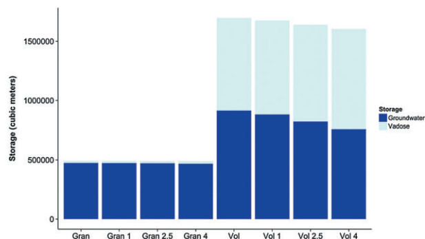
Figure 6. Average annual subsurface storage for the two hillslopes, compartmentalized by groundwater and vadose zone storage, for the base, warm, hot, and hotter scenarios
