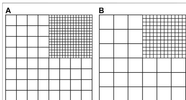
FIGURE 2 | Schematics of the high-granularity and low-granularity regions of the (A) electromagnetic and (B) hadron layers.
