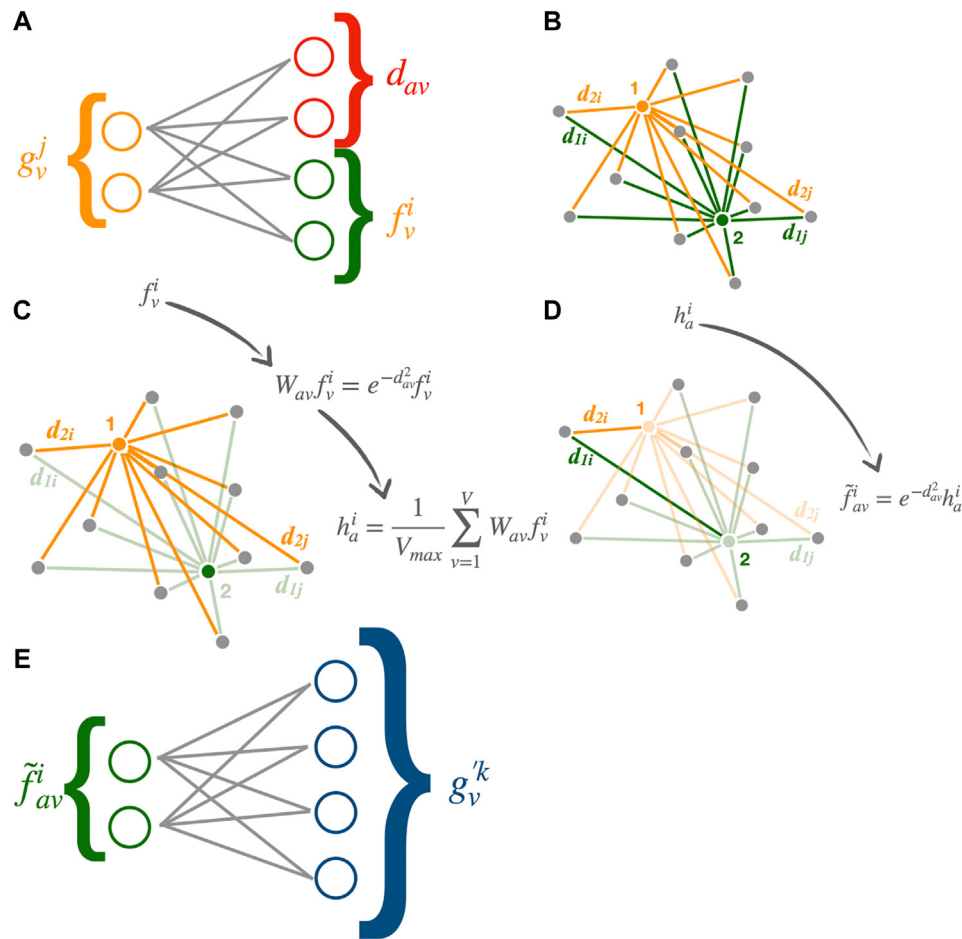
FIGURE 1 | Processing flow of the modified GARNET algorithm: (A) The input features ( g_v^j ) of each vertex are processed by a linear network, that returns a new set of features ( f_v^i ) and its distance from the S aggregators ( d_{av} ). (B) A graph is built in the learned space, using the d_{av} distances. (C) A message is gathered by each aggregator, as a weighted sum across the vertices of f_v^i , with W_{av} = \exp(-d_{av}^2) as weights. (D) A message from each aggregator ( \tilde{f}_{av}^i ) is passed back to each vertex, with the same W_{av} weight. (E) The aggregated outputs of each vertex are given as input to a neural network, which returns the learned representation.
