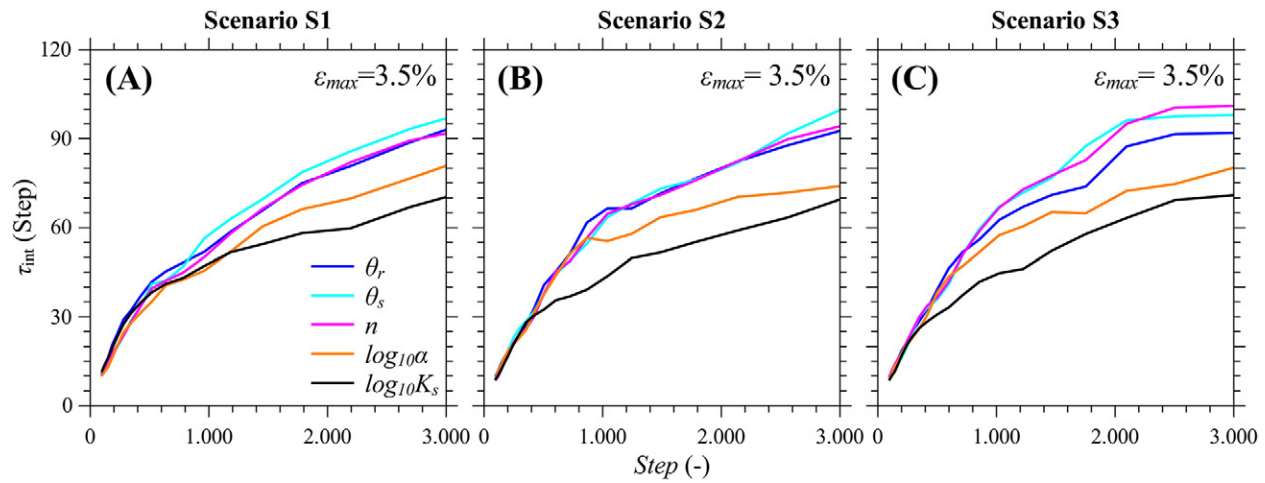
Fig. 3. The diagnostic plot of the Affine Invariant Ensemble Sampler (AIES) algorithm for synthetic modeling scenarios showing the integrated autocorrelation time \tau_{\text{int}} against the algorithm step for the soil hydraulic parameters of residual soil water content ( \theta_r ), saturated soil water content ( \theta_s ), the van Genuchten–Mualem parameters n and \alpha , and saturated hydraulic conductivity ( K_s ), along with the maximum statistical error ( \epsilon_{\text{max}} ) for Scenarios (A) S1, (B) S2, and (C) S3.
