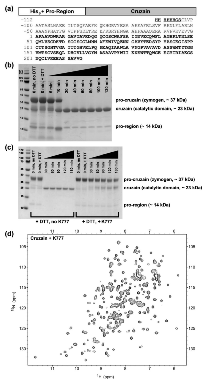
Figure 1. Domain diagram of cruzain, activation and inhibition of its zymogen form, and 15 N- 1 H HSQC spectrum (a) The domain diagram and one-letter sequence of the zymogen (pro-cruzin). The active catalytic domain (cruzain) used in this study is highlighted as boldface. Residues of an engineered N-terminal His 6 -tag (underlined) and the truncated pro-region are numbered -112 to -1. Residue numbers of cruzain are numbered 1 to 215. (b) Incubation at 37 °C and addition of DTT to PMSF- and MMTS-inhibited zymogen (~ 37 kDa) initiates auto-proteolysis of the N-terminal pro-region (~ 14 kDa) from the catalytically active domain (~ 23 kDa), as monitored by SDS-PAGE. (c) Addition of the vinyl sulfone K777 to pro-cruzin impedes, but does not completely inhibit, self-activation of the zymogen. (d) The 15 N- 1 H HSQC spectrum of cruzain inhibited with K777 indicates a well-folded and stable enzyme structure.
