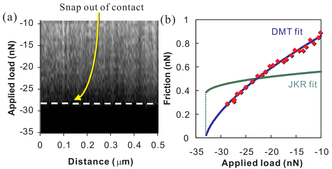
FIG. 2: (Color online) (a) Friction map as a function of applied load at 0V sample bias (scanning speed=500nm/s). (b) Plot of the friction force versus load at 0V sample bias.
