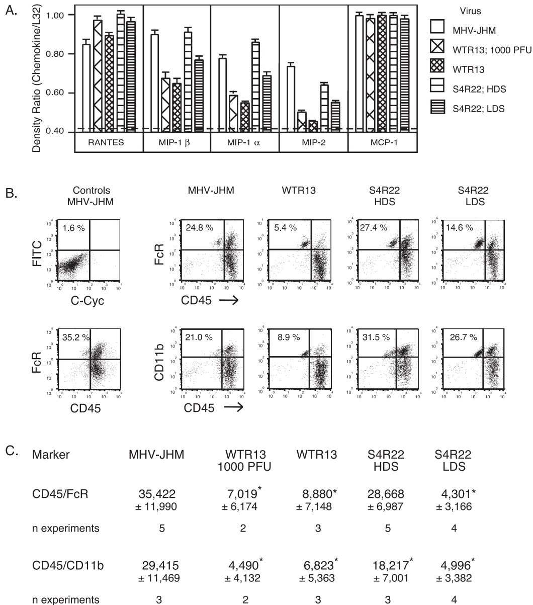
Fig. 5. The S gene of MHV-JHM enhanced macrophage inflammatory protein mRNA levels and macrophage infiltration into the CNS. Mice were infected with 10 PFU MHV-JHM, WTR13, and S4R22 unless otherwise indicated. (A) On day 7, brains were harvested and total RNA was isolated. Samples (4–10/group) were analyzed by RPA. Means \pm SE of band intensities normalized against L32 are shown. Sham infections resulted in background levels of chemokines, indicated by dashed line. (B) Mononuclear cells isolated from infected brains were co-stained for CD45/Fc \gamma R or CD45/CD11b. Percents shown indicate the percent of either CD45 high/Fc \gamma R high or CD45 high/CD11b high cells depicted in the upper-right hand quadrants of graphs. (C) The numbers of macrophages per brain were estimated as in Fig. 3. Means \pm SE of indicated number of experiments are shown. HDS, high disease score; LDS, low disease score. Statistical differences ( p < 0.05 ) between groups as indicated by *, such that groups with * are statistically different from groups without *. The non-statistical value difference between S4R22 CD45 high/CD11b high and cohort groups most likely reflects the lower n . Statistical analysis was performed by one-way ANOVA.
