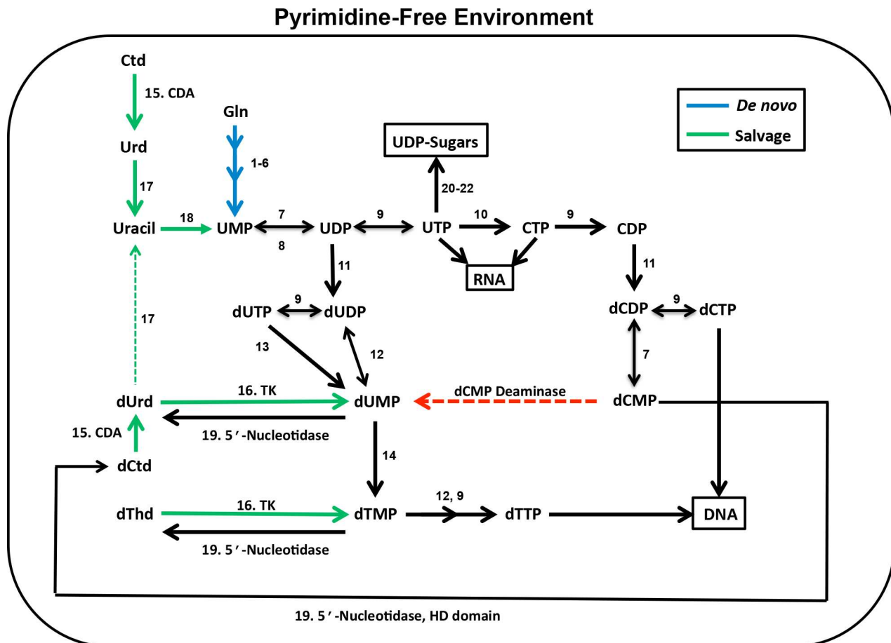
Fig 1. T. brucei pyrimidine pathway. Green lines salvage routes, blue lines de novo pathway, black lines interconversion routes, and the red dotted line indicates a reaction that is not present in trypanosomatids. The numbers above each arrow represent the enzyme catalyzing the reaction (EC number): 1–6 : carbamoyl phosphate synthase (6.3.5.5), aspartate carbamoyl transferase (2.1.3.2), dihydroorotase (3.5.2.3), dihydroorotate dehydrogenase (1.3.98.1), orotate phosphoribosyltransferase (2.4.2.10), orotidine 5-phosphate decarboxylase (4.1.1.23); 7 UMP-CMP kinase (2.7.4.14); 8 : nucleoside diphosphatase (3.6.1.6); 9 : nucleoside diphosphate kinase (2.7.4.6); 10 : cytidine triphosphate synthase (6.3.4.2); 11 : ribonucleoside diphosphate reductase (1.17.4.1); 12 : thymidylate kinase (2.7.4.9); 13 : deoxyuridine triphosphatase (dUTPase) (3.6.1.23); 14 : dihydrofolate reductase-thymidylate synthase (2.1.1.45); 15 : cytidine deaminase (CDA) (3.5.4.5); 16 : thymidine kinase (TK) (2.7.1.21); 17 : uridine phosphorylase (2.4.2.3); 18 : uracil phosphoribosyltransferase (2.4.2.9); 19 : HD-domain 5'-nucleotidase (3.1.3.89); 20 : UDP-glucose pyrophosphorylase (2.7.7.9); 21 : UTP N-acetyl- \alpha -D-glucosamine-1-phosphate uridylyltransferase (2.7.7.23); 22 : UDP-glucose 4-epimerase (5.1.3.2). The pathway was constructed based on the annotation described in [10] and modified to incorporate results from our studies. Additionally enzyme 7 was added based on the published report that one of seven encoded adenylate kinases (ADKG) was biochemically characterized and shown to be a UMP-CMP kinase [16].
