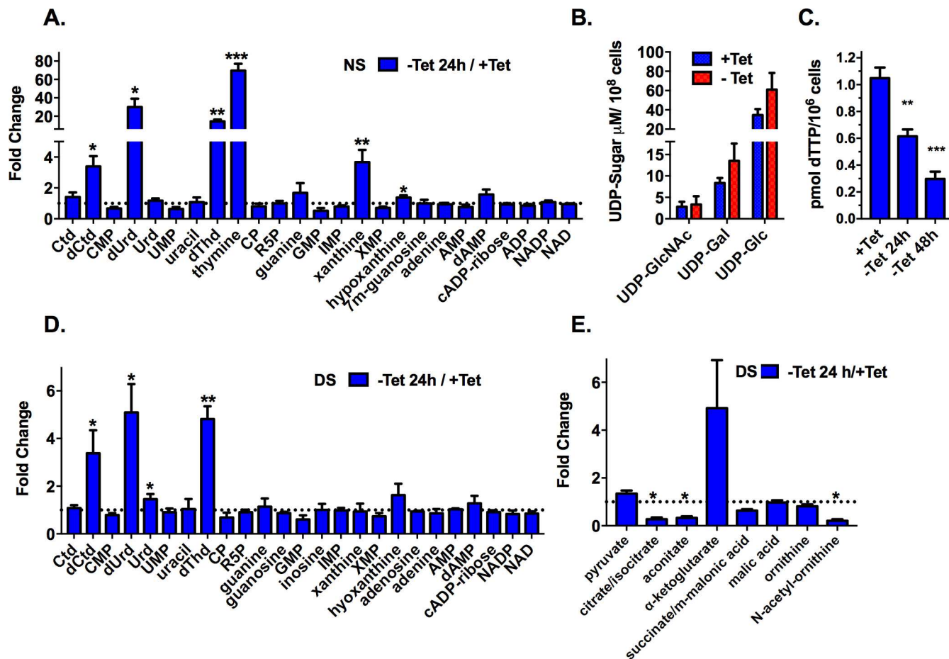
Fig 6. Metabolomic analysis of TK c-null cells. A. Detected pyrimidine and purine bases, nucleosides and nucleotides for cells grown in HMI-19 medium supplemented with normal serum (NS). The ratios (fold change) of metabolite levels in the absence of Tet for 24h compared to cells grown with Tet are plotted. B. HPAEC analysis of nucleotide sugars \pm Tet at 24 h. C. Quantitation of dTTP by enzymatic assay \pm Tet at 24 and 48 h for cell grown in HMI-19 supplemented with NS. D. Fold change of detected pyrimidine and purine bases, nucleosides and nucleotides \pm Tet at 24 h for cells grown in HMI-19 medium supplemented with dialyzed serum (DS). E. Fold change of TCA intermediates \pm Tet at 24 h for cells grown in HMI-19 medium supplemented with DS. Metabolites shown for C and D are from the same experiment. Data for additional detected metabolites for the normal serum (A) and dialyzed serum (D and E) studies are presented in Supplemental Figures. All data were collected in biological triplicate and error bars represent the SEM calculated for the \pm Tet ratio by Graph Pad Prism using the baseline-correction algorithm. For A, D and E, multiple T test analysis was performed in GraphPad Prism comparing the +Tet and -Tet conditions for each study. Statistical significance was determined without correction for multiple comparisons and without assuming a consistent standard deviation. For C, data were analyzed using one way ANOVA with Dunnett's multiple comparison test. Metabolites that showed a significant difference between the conditions are marked * P < 0.05 , ** P < 0.01 , *** P < 0.001 . Abbreviations are common nomenclature or have been previously defined except for CP, carbamoyl phosphate, R5P, ribose 5'-phosphate, 7m-guanosine, 7-methyl guanosine, succinate/m-malonic acid, succinate/methyl-malonic acid.
