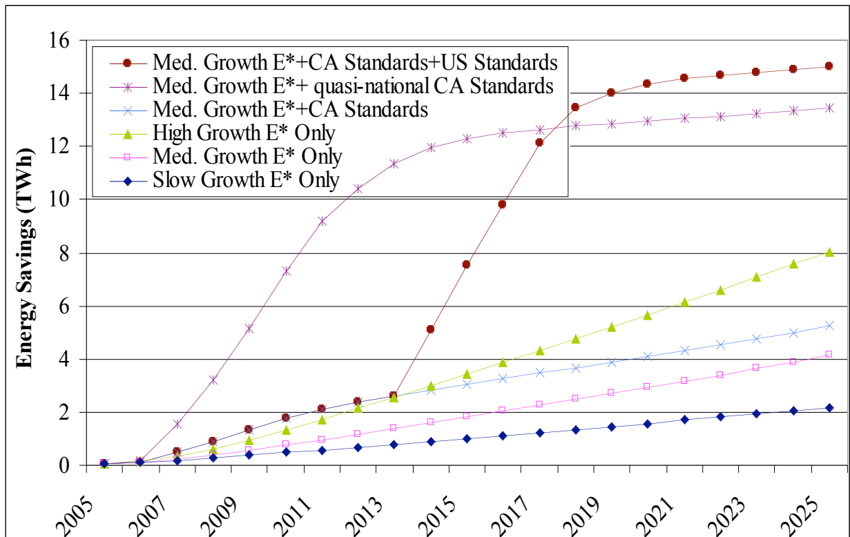
Figure 7. Energy Savings for External Power Supplies (TWh)
