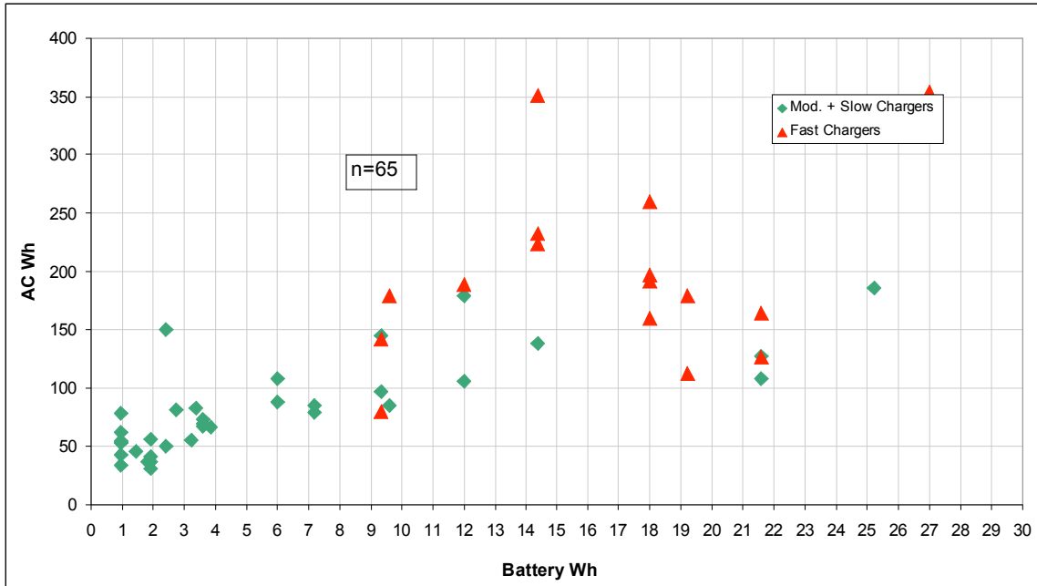
Figure 3. AC Energy Use Graphed on DC Battery Capacity
