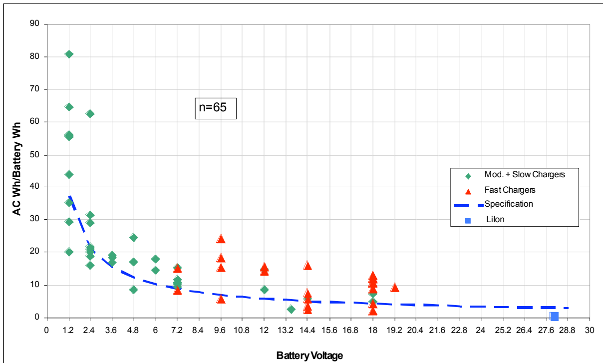
Figure 4. Specification: Energy Use Ratio Graphed on Battery Voltage
