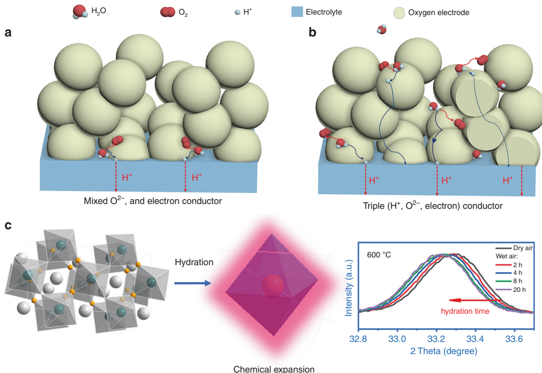
Fig. 1 Water splitting reaction on oxygen electrode and PNC's hydration. a Mixed oxygen-ion O 2- and electron conducting electrode. b Triple (H + , O 2- , and electron) conducting electrode to extend reaction to entire electrode surface. c Chemical expansion of PNC perovskite structure observed in high-temperature X-ray diffraction at 600 °C when exposed to wet air.
