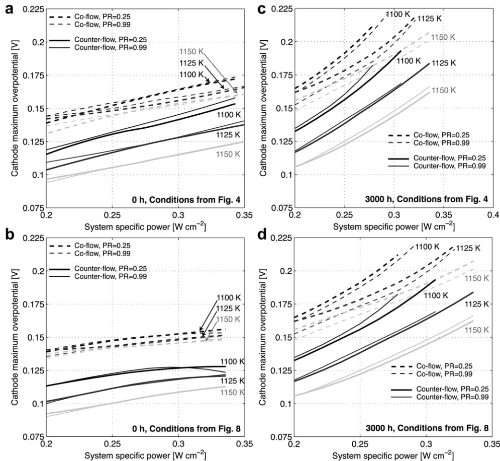
Fig. 12. Maximum local cathode overpotential at the initial time (a, b) and after 3000 h of operation (c, d) at a constant system power (c, d), under the conditions depicted in Figs. 4 and 8, for the co-flow (dashed lines) or counter-flow (solid lines) configuration, with different discrete maximum allowable cell temperatures (grayscale variations) and methane conversion fraction in the reformer (line thickness). The largest discrepancy between the trend line and the actual result is 6.5%.
