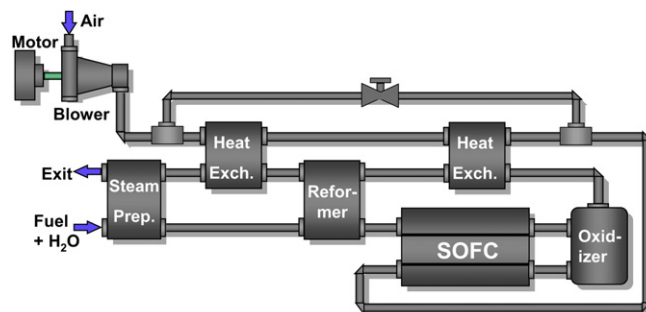
Fig. 2. Schematic view of a typical layout of SOFC system for CHP application.
