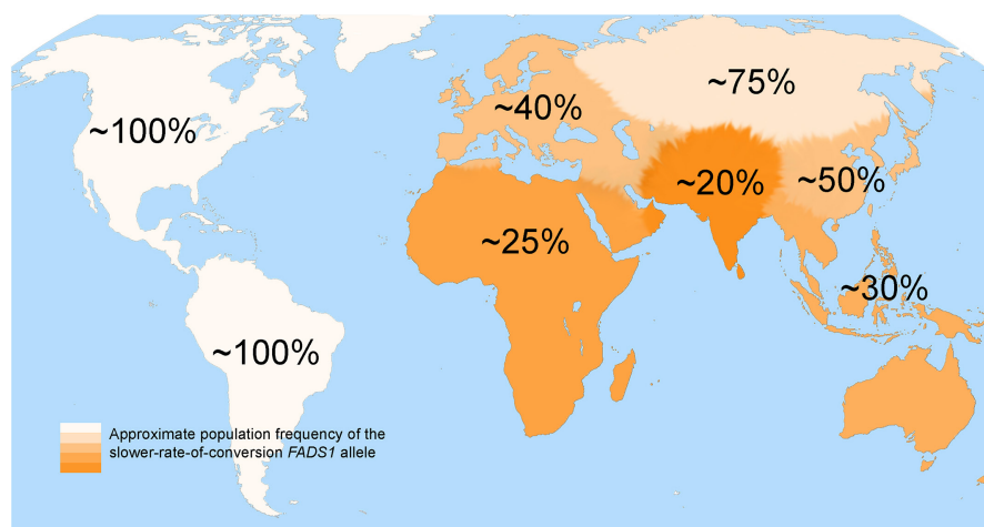
FIGURE 1 Map showing world-wide occurrence of the slower rate-of-conversion FADS variant. The population-level frequencies reported here are estimated from Mathieson and Mathieson (2018) 8
