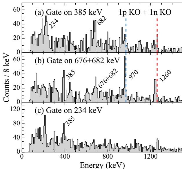
FIG. 7. (Color online) Coincidence spectra for the 385-keV, the 676-682 keV doublet, and the 234-keV transitions from the sum of the one-proton and one-neutron knockout reaction channels. Due to low statistics, the placement of the 385-keV transition remains tentative. The displacement of the yrast energies in panel (b), as indicated by the dashed lines at the expected yrast energies, is discussed in the text.
