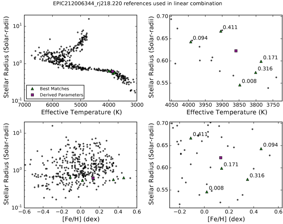
Figure 4. SpecMatch-Emp characterization of EPIC212006344. Black points: T_{\text{eff}} , R_* , and [\text{Fe}/\text{H}] from the SpecMatch-Emp library. Green triangles: properties of the closest-matching library spectra (red spectra in Figure 3). Purple square: linear combination of library spectra spectra. The final derived parameters are T_{\text{eff}} = 3925 \pm 70 K, [\text{Fe}/\text{H}] = 0.43 \pm 0.12 dex, R_* = 0.63 \pm 0.10 dex.
