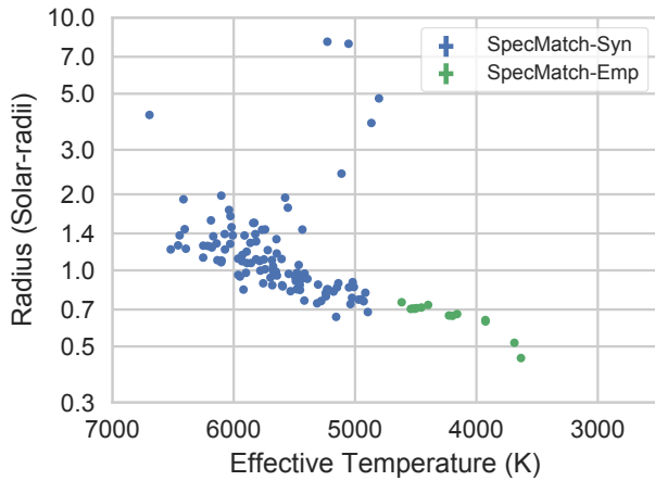
Figure 5. K2OIs with reliable effective temperatures and stellar radii, as measured by SpecMatch-Syn (blue) or SpecMatch-Emp (green). Median uncertainties are shown at top right.
