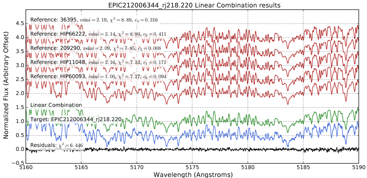
Figure 3. Example HIRES characterization spectrum with SpecMatch-Emp fit. Blue spectrum is of EPIC212006344, an M0 dwarf, and illustrates the typical SNR from our characterization program of \approx 45/\text{pixel} . The spectrum contains a dense forest of molecular lines, making ab initio spectral synthesis challenging. Red spectra are drawn from SpecMatch-Emp library and are identified as similar to the target spectrum by the SpecMatch-Emp algorithm. The green and black spectra are the best-fitting linear combination spectrum and residual spectrum, respectively.
