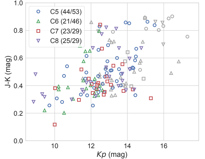
Figure 2. Distribution of K2OIs as a function of Kp and J-K color. The colored/gray points represent targets with/without a HIRES spectrum. The marker color and shape represent a target’s specific K2 campaign. The HIRES follow-up is nearly complete to Kp = 14 mag.
