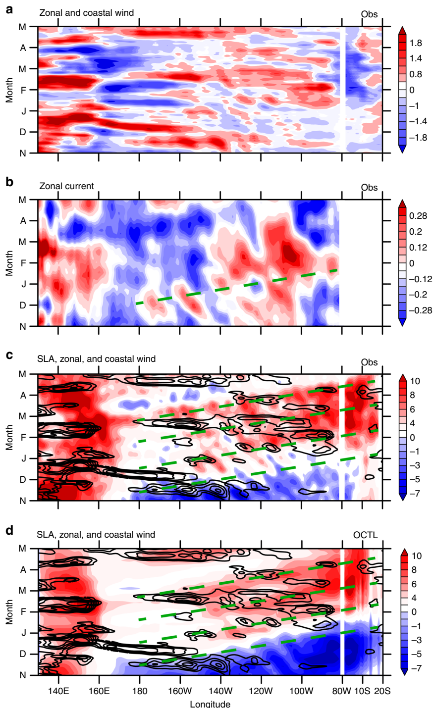
Fig. 4 Longitude-time evolution of the 2017 extreme coastal El Niño. Hovmöller diagrams for: a zonal and coastal wind anomalies (color shading; m s -1 ; negative values along the coast of South America indicates northerly wind anomalies); b zonal current (color shading; m s -1 ), green dashed line indicates Kelvin wave propagation; c SLA (color shading; cm) and zonal wind anomalies (contours with an interval of 0.5 m s -1 ; positive solid and negative omitted) from observations; d same as c but from MITgcm OCTL. All meridionally averaged in 2°S–2°N along the equator and zonally averaged in 80°W–85°W along the coast
