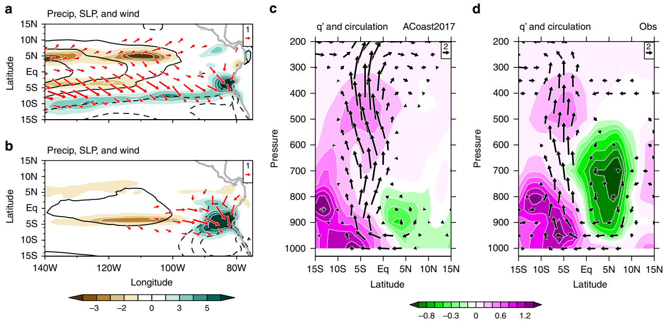
Fig. 7 Atmospheric response to 2017 FMA SSTAs. The 10-year-mean anomalies of FMA precipitation (color shading; \text{mm day}^{-1} ), sea level pressure (contours at an interval of 10 hPa, zero omitted, and negative dashed), and surface wind anomalies (vectors; \text{m s}^{-1} ) for a A2017 and b ACoast2017. Vertical circulation anomalies (vectors; \text{m s}^{-1} ) and specific humidity ( q' , \text{g kg}^{-1} ; color shading) along the west coast of America based on c ACoast2017 and d observations (zonally averaged in 80^\circ\text{W} – 85^\circ\text{W} )
