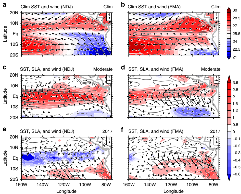
Fig. 8 Ocean-atmospheric conditions of basin-scale moderate El Niño and the 2017 extreme coastal El Niño. Climatological SST ( ^\circ\text{C} ; color shading; 27 and 28^\circ\text{C} contours in gray line) and winds (vectors; \text{m s}^{-1} ) over the eastern Pacific for a NDJ and b FMA; composite NDJ (left) and FMA (right) SSTAs ( ^\circ\text{C} ; color shading), SLA (contours with an interval of 2 cm, zero omitted and negative dashed) and wind anomalies ( \text{m s}^{-1} ; arrows) for basin-scale moderate El Niño ( c , d ) and the 2017 extreme coastal El Niño ( e , f )
