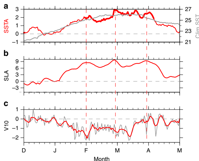
Fig. 3 Evolution of the 2017 extreme coastal El Niño. Time series of a climatological SST ( ^{\circ}\text{C} ; gray line) and SSTA ( ^{\circ}\text{C} ; red line), the bold red line indicates SSTs above 27^{\circ}\text{C} ; b SLA (cm) and c meridional alongshore wind anomalies ( \text{m s}^{-1} ; gray line is obtained from raw data and red line indicates 5-day running mean result). SSTs and winds are averaged in CTSA while SLA is averaged in 85^{\circ}\text{W}–95^{\circ}\text{W} , 2^{\circ}\text{S}–2^{\circ}\text{N} to measure equatorial waves in the eastern Pacific
