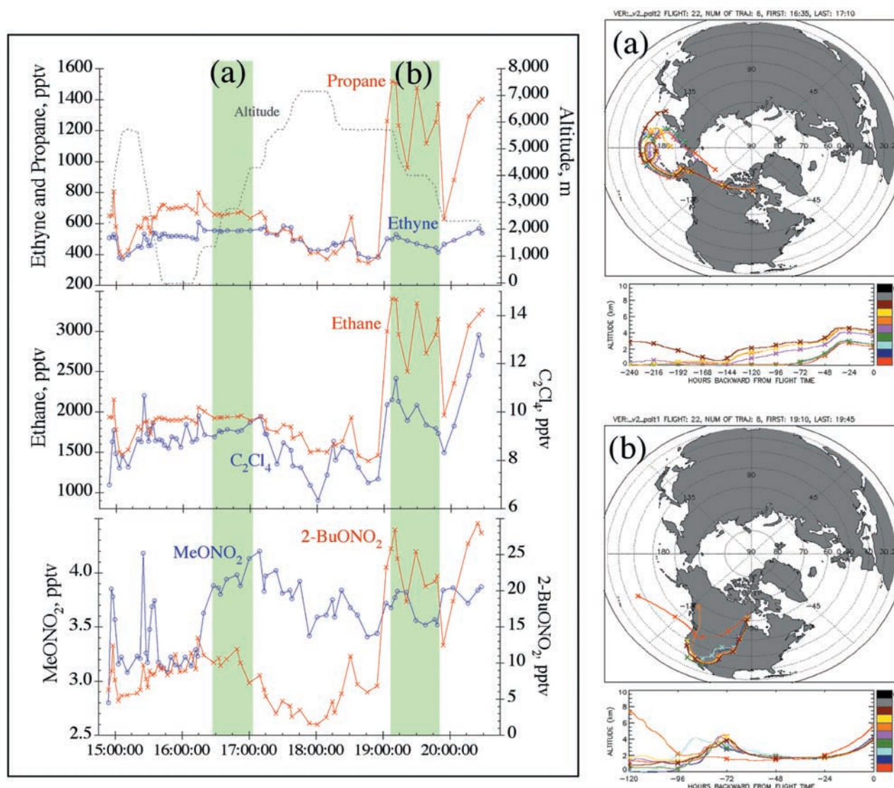
Figure 21. Altitude, propane, ethyne, ethane, C_2Cl_4 , methyl nitrate, and 2-butyl nitrate versus time for Flight 22, Thule to Churchill, 24 March 2000 (deployment 4). Also shown are back-trajectories showing the origins of the air masses sampled during the highlighted sections (a) and (b) of the flight.
