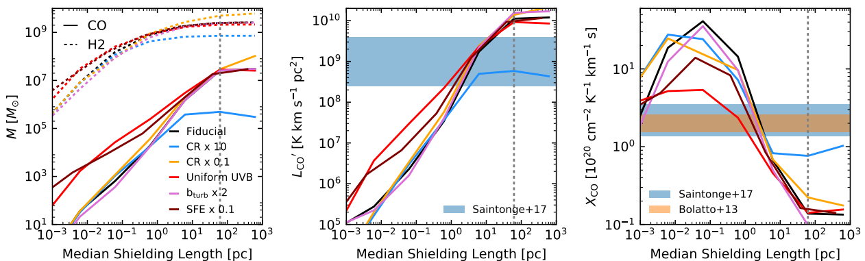
Figure 10. The effects of the changing the shielding length on the CO and H 2 masses (left), the CO(1-0) luminosity (middle) and the emission-weighted CO-to-H 2 conversion factor (right). The grey dotted vertical line shows the median of the original distribution of Sobolev lengths plus local cell correction. The black lines are the same as the black points in Figure 6. The other coloured lines show the effects of changing different assumptions in our modelling: increasing the cosmic ray ionization rate by a factor 10 (blue line), lowering the cosmic ray ionization rate by a factor 10 (orange line), using a homogeneous UV background set to the interstellar radiation field from Black (1987) (red line), increasing the subgrid turbulence in our model by a factor 2 (pink line) and restarting the simulation with a lower local star formation efficiency to allow more dense gas to build up (maroon line). We compare with the observations from the xCOLD GASS survey (Saintonge et al. 2017) and Bolatto et al. (2013).
