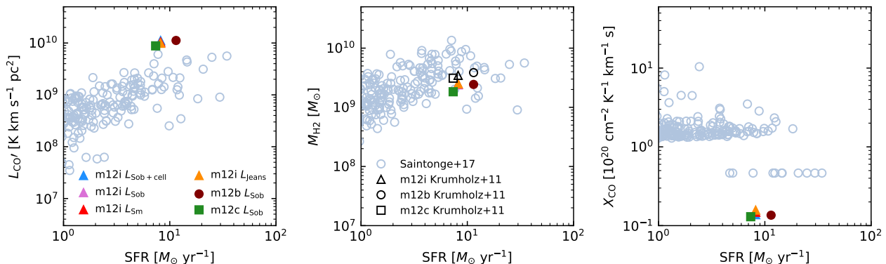
Figure 4. CO(1-0) luminosity (left), H 2 gas mass (middle) and CO-to-H 2 conversion factor (right) at a given star formation rate. Plotted in light blue are the observations from the xCOLD GASS sample (Saintonge et al. 2017) assuming the metallicity-dependent CO-to-H 2 conversion factor from Accurso et al. (2017). The blue, orange, red and pink triangles show the results for the m12i galaxy assuming different shielding lengths. Note that these points overlap with each other almost perfectly. The brown circle and green square show results from other simulations, assuming the Sobolev shielding length plus a contribution from the local cell. In the middle panel, the black open points are obtained from calculating the H 2 fraction for each particle using the Krumholz & Gnedin (2011) fitting function (which is used to determine the molecular fraction of gas in FIRE-2).
