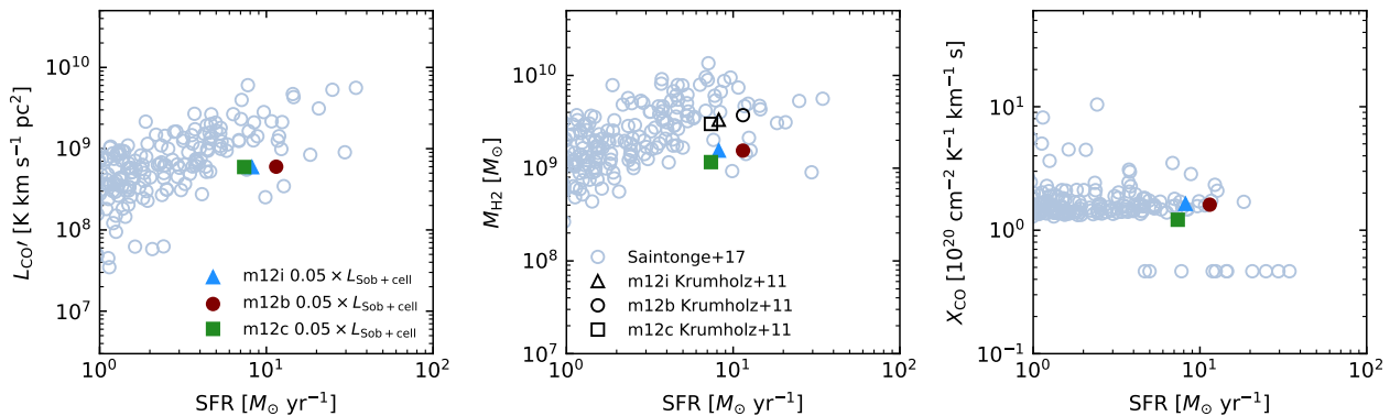
Figure 9. CO(1-0) luminosity (left), H 2 gas mass (middle) and CO-to-H 2 conversion factor (right) at a given star formation rate. Plotted in light blue are the observations from the xCOLD GASS sample (Saintonge et al. 2017) assuming the metallicity-dependent CO-to-H 2 conversion factor from Accurso et al. (2017). The coloured points are results from the simulations all assuming that the distribution of Sobolev shielding lengths plus local cell correction has been rescaled by a constant factor of 0.05, corresponding to a median length of 3 pc for cold ( T < 300 K) gas. In the middle panel, the black open points are obtained from calculating the H 2 fraction for each particle using the Krumholz & Gnedin (2011) fitting function.
