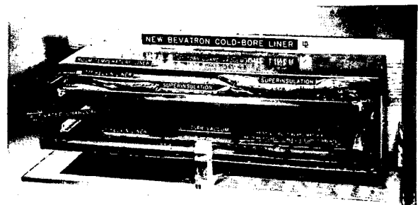
Fig. 6. Cross section of the new vacuum liner installed in the Bevatron. This cryogenically-cooled fiberglass assembly brings the average pressure in the beam path down to the low- 10^{-10} Torr range.
