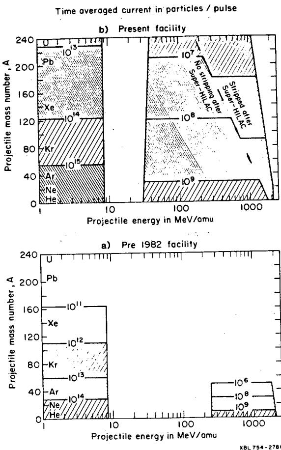
Fig. 3. Ion and beam intensity capabilities of the Bevalac; a) prior to the U-Beams Project and b) after the upgrade. SuperHILAC intensities (on the left side of the figure) are in particles-per-second, Bevalac numbers are in particles-per-pulse.
