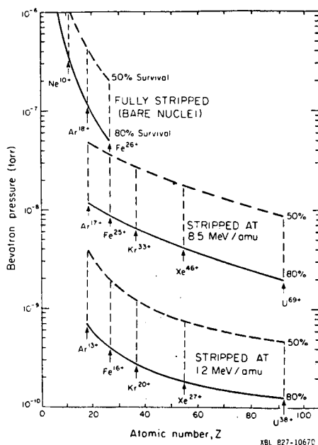
Fig. 5. Vacuum requirements for beam survival in the Bevatron. Most stringent requirements are for ions not stripped at the SuperHILAC exit.
