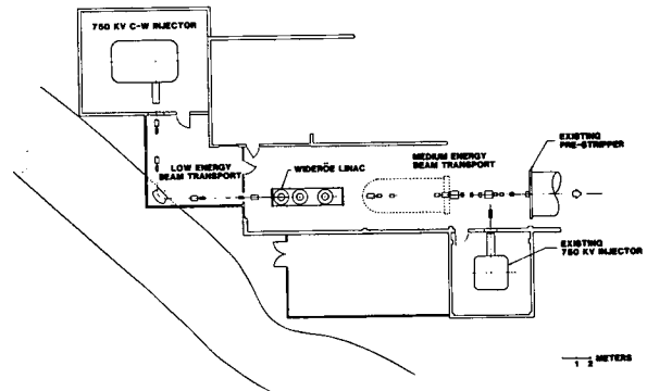
Fig. 4. Plan view of the new ABEL injector at the SuperHILAC.
