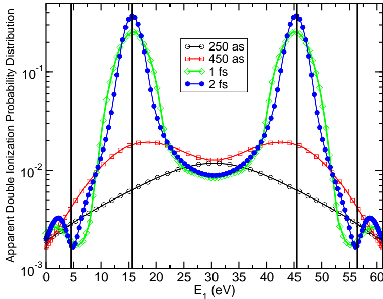
Figure 4. (Color online) Calculated electron energy distributions for pulse duration of 250 as, 450 as, 1 fs and 2 fs at 70 eV and I=10^{12} W cm ^{-2} , showing the peaks due to ionization via the n = 2 states of He ^{+} that shift with pulse duration.
