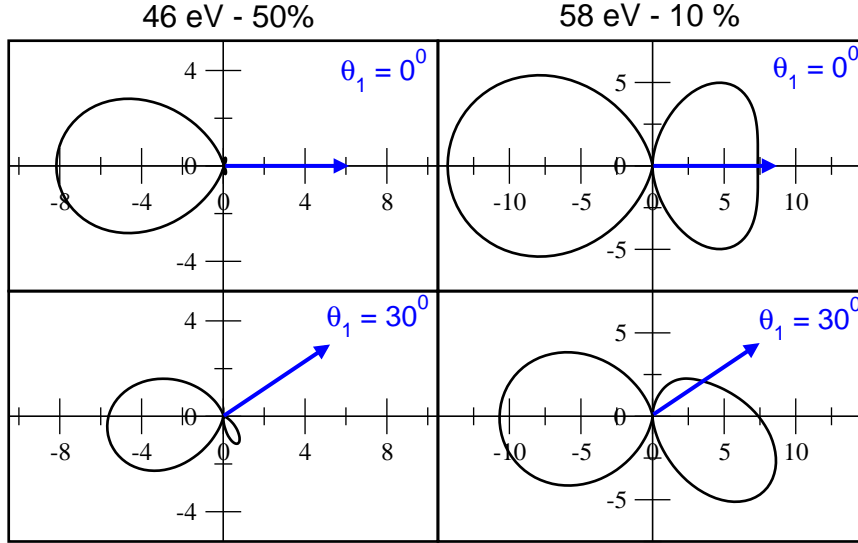
Figure 5. (Color online) Angular distributions at 46 eV photon energy with 50% energy sharing (left column) and 58 eV with 10% energy sharing (right column). Each row corresponds to a different angle of one electron fixed with respect to the polarization vector (horizontal axis). Results are shown for a pulse duration of one fs and calculated with l_{max} = 7 .
