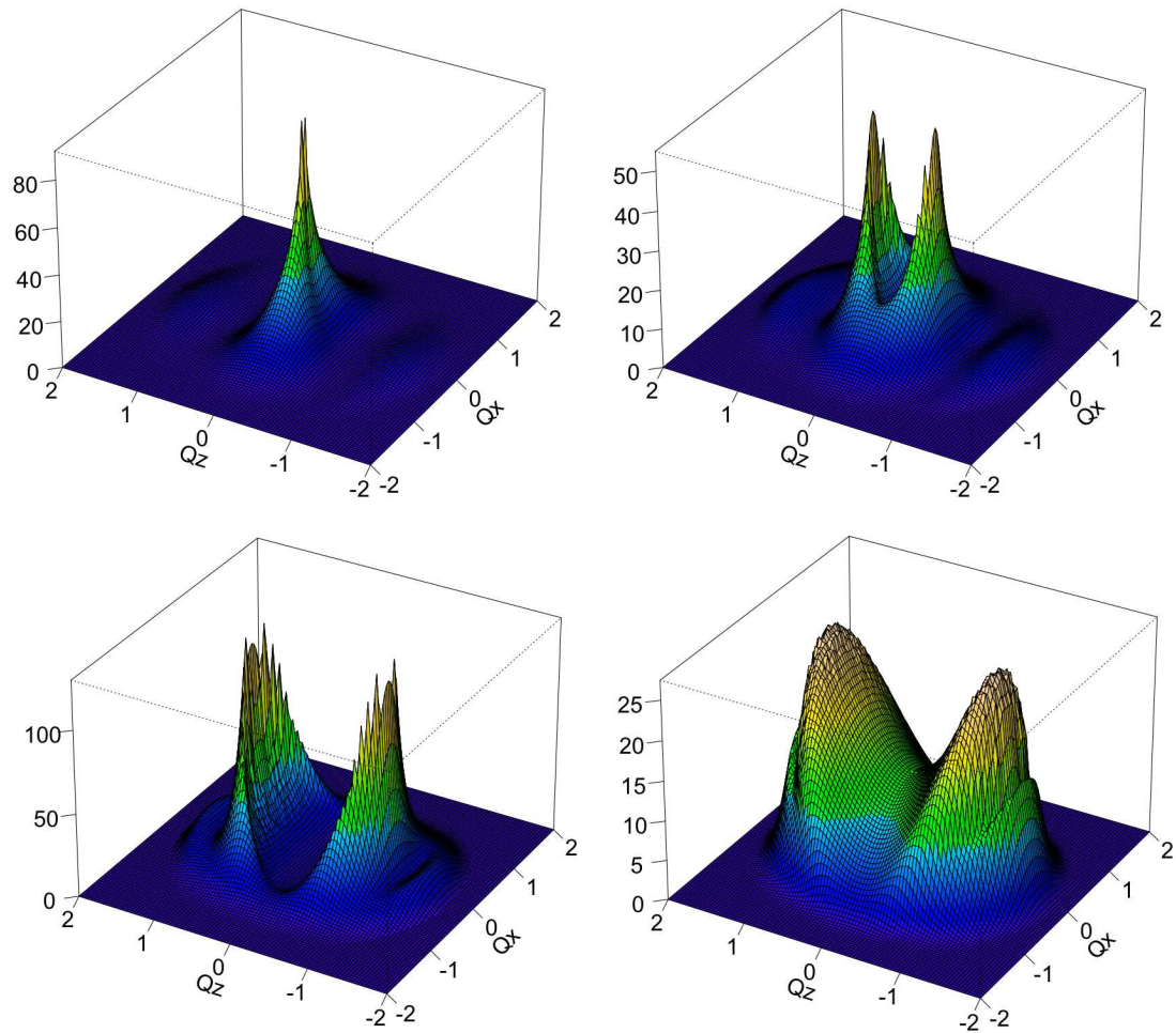
Figure 7. (Color online.) Nuclear recoil momentum distributions, integrated over Q_y , at 52 eV photon energy for calculations using a 2 fs pulse. Polarization is along the z-axis. Energy sharings, left to right: top row, 50%, 70%; bottom row, 90%, integrated over energy sharing.
