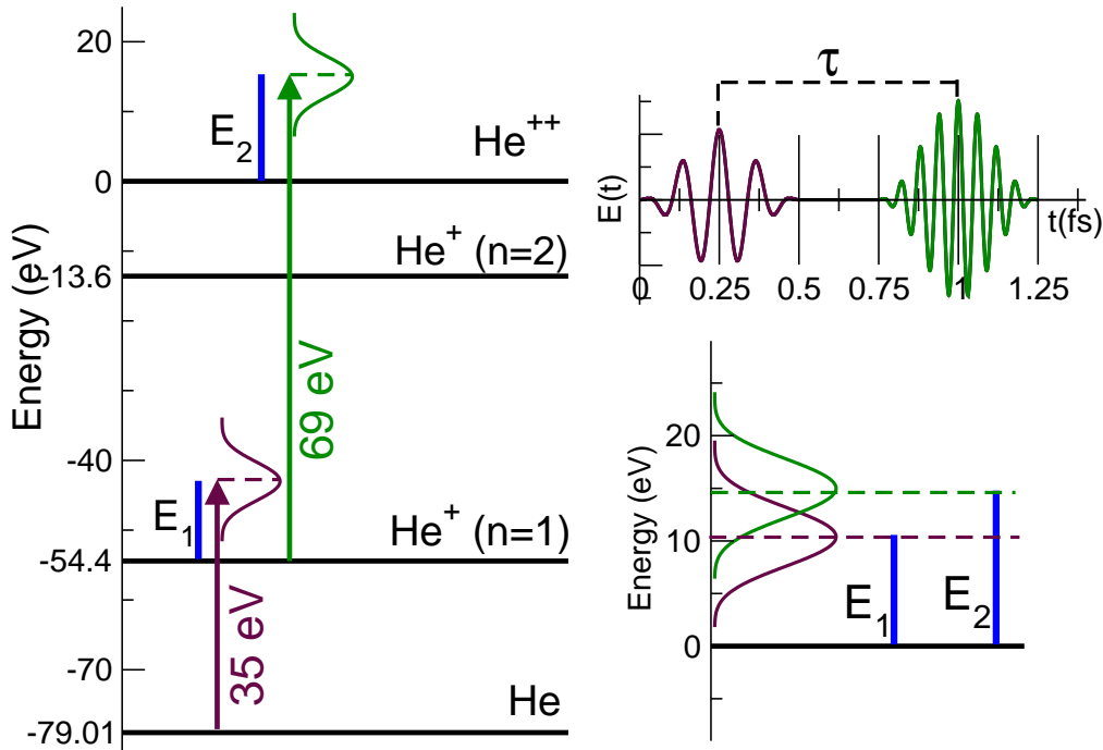
Figure 8. (Color online.) Left: Schematic of the energetics for a two-color two-photon double ionization process in helium. Top Right: Electromagnetic field as function of time showing two pulses of 500 as, with 35 and 69 eV respectively and a time delay of \tau = 750 as between them. Bottom right: Expected energies for electrons ejected from each sequential process.
