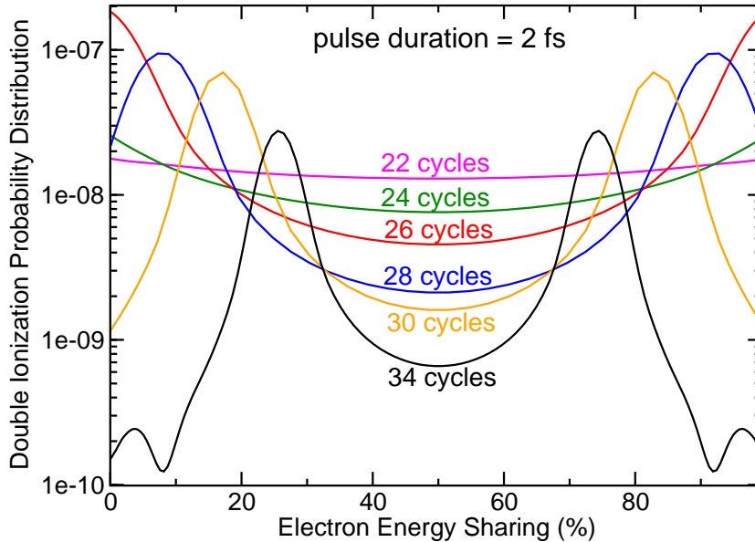
Figure 3. (Color online) Electron energy distributions for a fixed pulse duration of 2 fs and intensity of 10^{12} W cm ^{-2} at different photon energies. Plotted energies go from below the first sequential threshold to above the second sequential threshold: 22 cycles (45.5 eV), 24 cycles (49.63 eV), 26 cycles (53.8 eV), 28 cycles (57.9 eV), 30 cycles (62.05 eV) and 34 cycles (70.3 eV).
