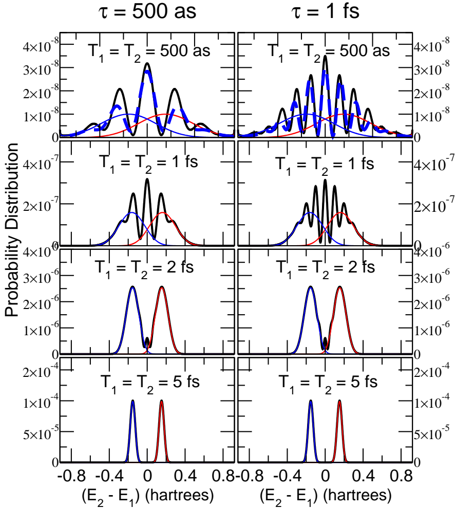
Figure 10. (Color online.) Electron energy joint distributions determined at the central energies of the pulses. Left column: delay of 500 as. Right column: delay of 1 fs. Each row corresponds to different pulse durations (in all cases both pulses have same pulse duration). Black full lines: results obtained with the model (see text). Full thin curves are the squared values of J_i defined in Eq. (18) whose energy overlapping leads to the interference fringes. Dashed lines: ab initio calculations.
