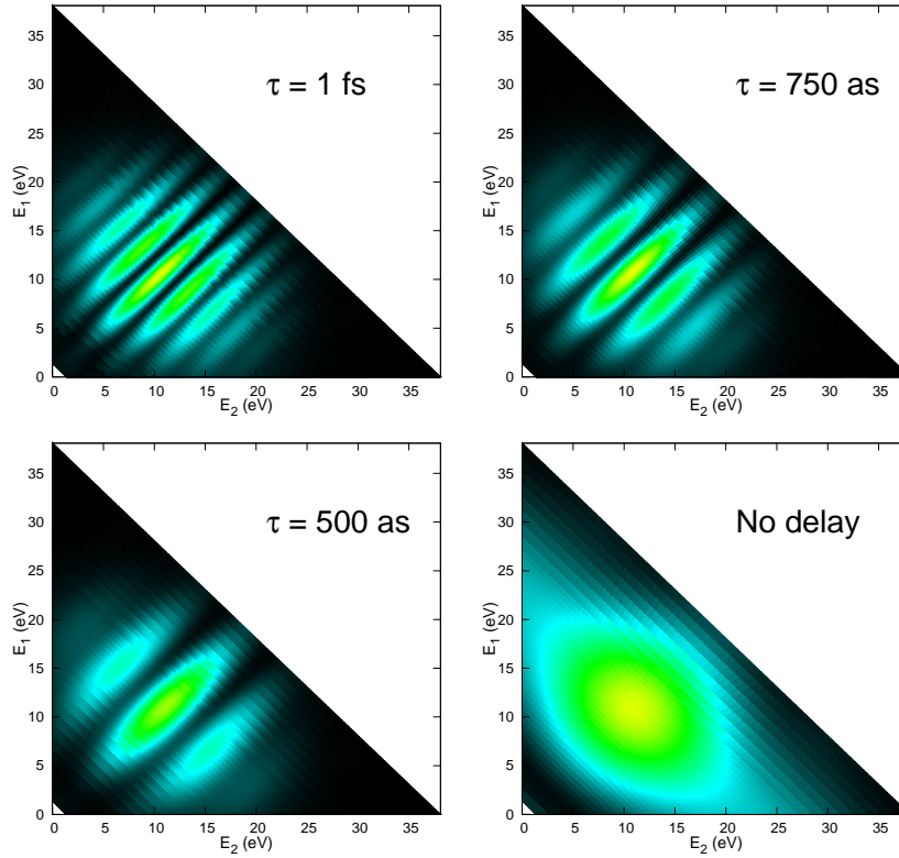
Figure 9. (Color online.) Joint electron energy distributions for pulse durations T_1 = T_2 = 500 as. Each panel corresponds to a different time delay between pulses.
