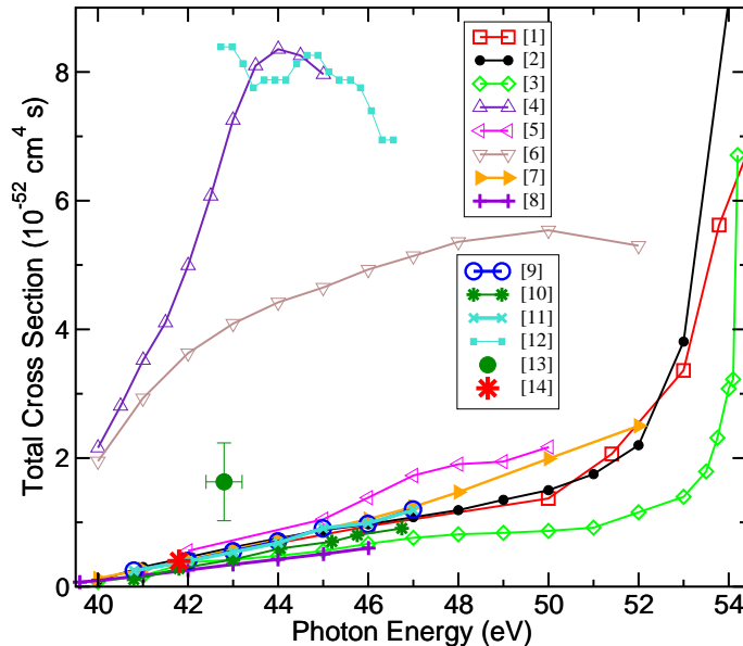
Figure 1. (Color online) Total two-photon double ionization cross sections as a function of photon energy. [1] 2fs results (Palacios et al. 2009a); [2] (Feist et al. 2008); [3] (Horner et al. 2007); [4] (Nikolopoulos & Lambropoulos 2007); [5] (Ivanov & Kheifets 2007); [6] (FC) (Foumouo et al. 2006); [7] (NC) (Foumouo et al. 2006); [8] (Hu et al. 2005); [9] (Piroux et al. 2003); [10] (Feng & van der Hart 2003); [11] (Laulan & Bachau 2003); [12] (Nikolopoulos & Lambropoulos 2001); [13] (Sorokin et al. 2007); [14] (Hasegawa et al. 2005).
