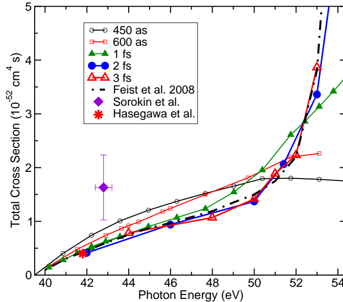
Figure 2. (Color online) Total two-photon double ionization cross sections as a function of photon energy. The current results are labeled with the corresponding pulse durations.
