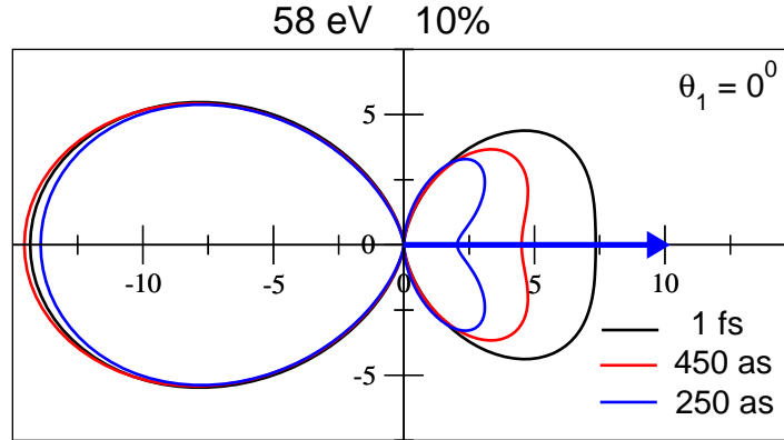
Figure 6. (Color online) Angular distributions from calculations including up to l_{max} = 7 for a photon energy of 58 eV with energy sharing of 10% and pulse lengths of 1 fs, 450 as and 250 as. Note that the all cross sections are normalized to the 1 fs TDCS for easier comparison of the shapes.
