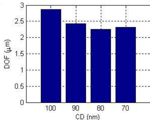
Fig. 10. DOF as a function of CD for isolated line features using the same criteria as used in Fig. 7
