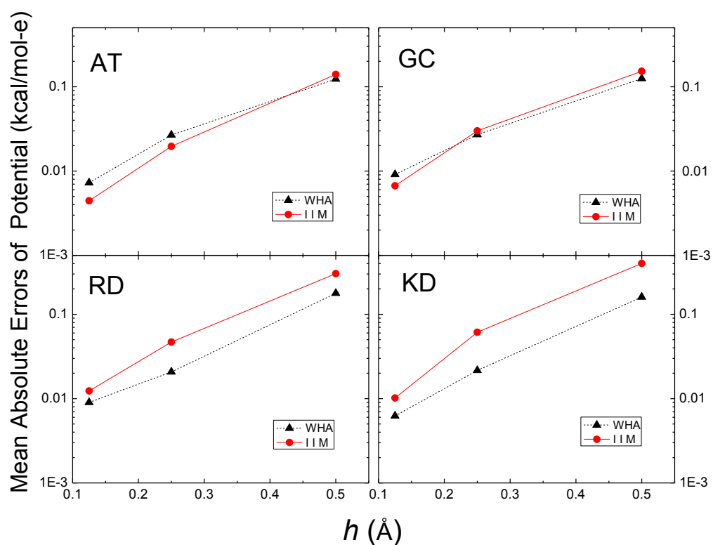
Figure 2. Mean absolute errors of reaction field potentials at the 8 nearest finite-difference grid points of each atom (kcal/mol-e) versus grid spacing h (Å) with respect to those calculated at the fine grid spacing of 1/16\text{Å} for AT, GC, RD and KD dimers, respectively.
