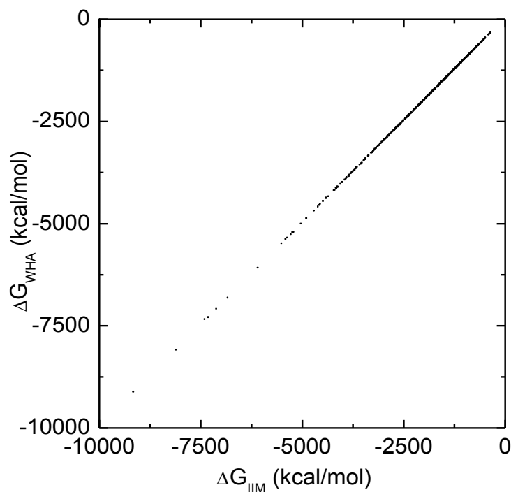
Figure 1. Correlation of reaction field energies ( \Delta G ) by IIM and WHA at 1/2 \text{ \AA} grid spacing for the Amber training set of 579 biomolecules. The Pearson correlation coefficient is 1.0000 and the linear regression slope is 1.0014 (with fixed offset of zero).
