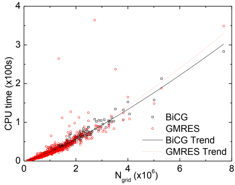
Figure 8. CPU time versus the number of grids ( N_{grid} ) for GMRES and BiCG, respectively. Convergence criterion (relative) is set to be 10^{-6} .
