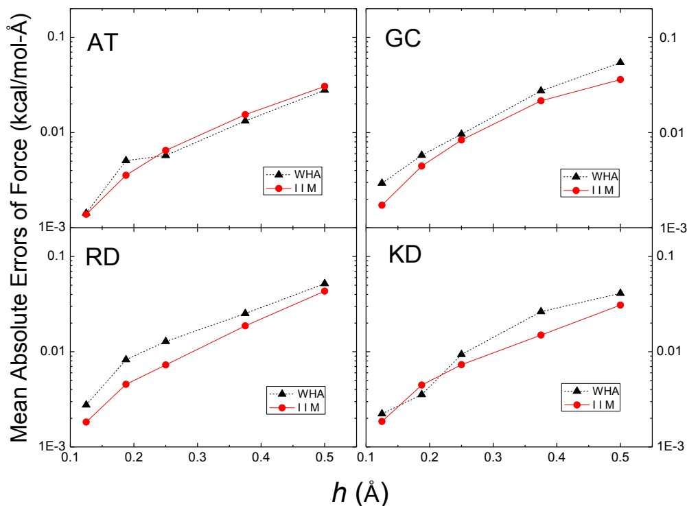
Figure 4. Mean absolute errors of reaction field forces at each atom ( \text{kcal/mol}\cdot\text{\AA} ) versus grid spacing h ( \text{\AA} ) with respect to those calculated at the fine grid spacing of 1/16\text{\AA} for AT, GC, RD and KD dimers, respectively.
