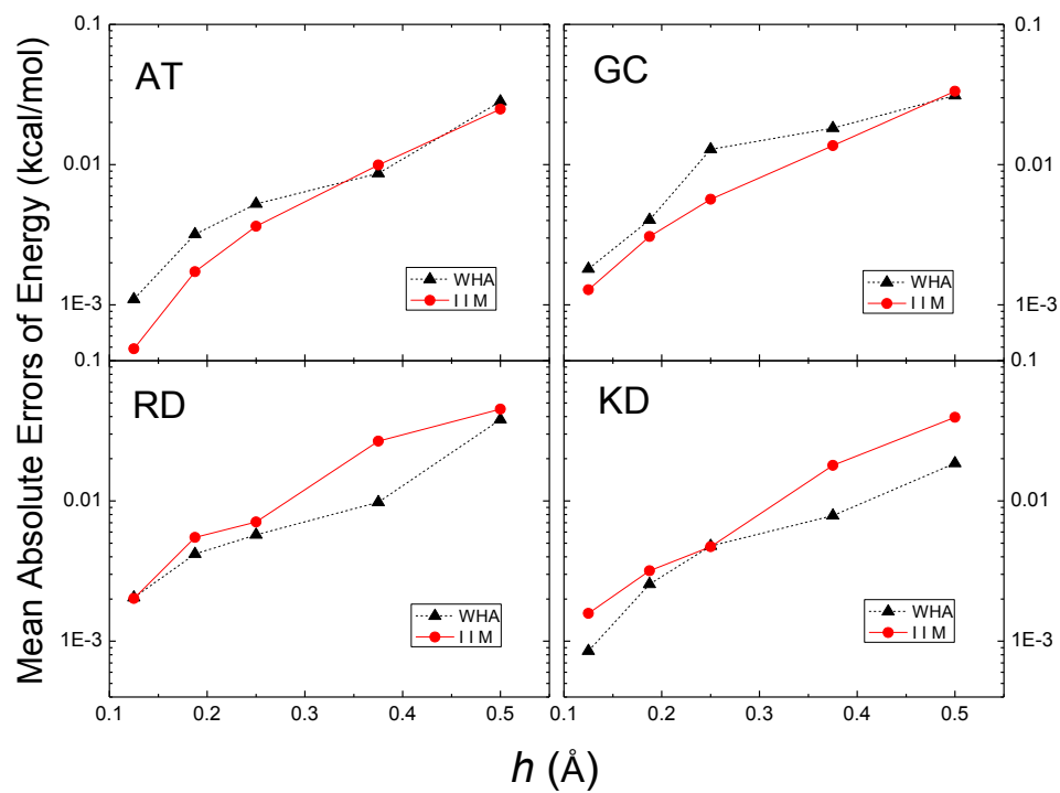
Figure 3. Mean absolute errors of reaction field energies at each atom (kcal/mol) versus grid spacing h (Å) with respect to those calculated at the fine grid spacing of 1/16 Å for AT, GC, RD and KD dimers, respectively.
