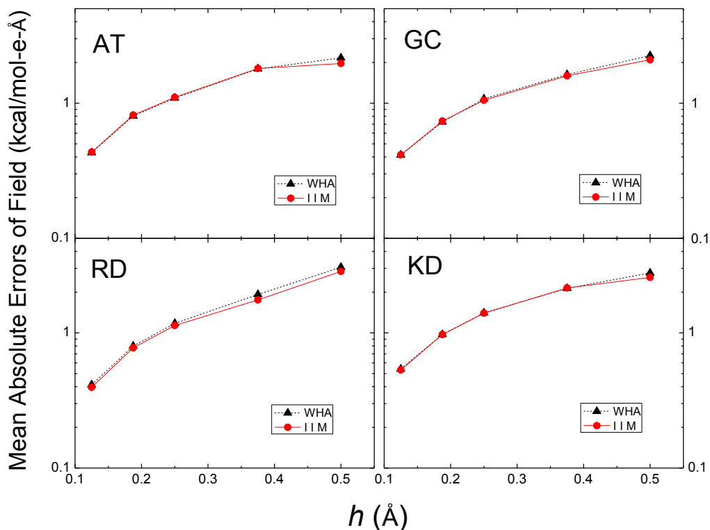
Figure 7. Mean absolute errors of reaction fields on the molecular surface (inside, kcal/mol-e-Å) versus grid spacing h (Å) with respect to those calculated at the fine grid spacing of 1/16\text{Å} for AT, GC, RD and KD dimers, respectively. A second-order least square fitting method was used in all tests.
