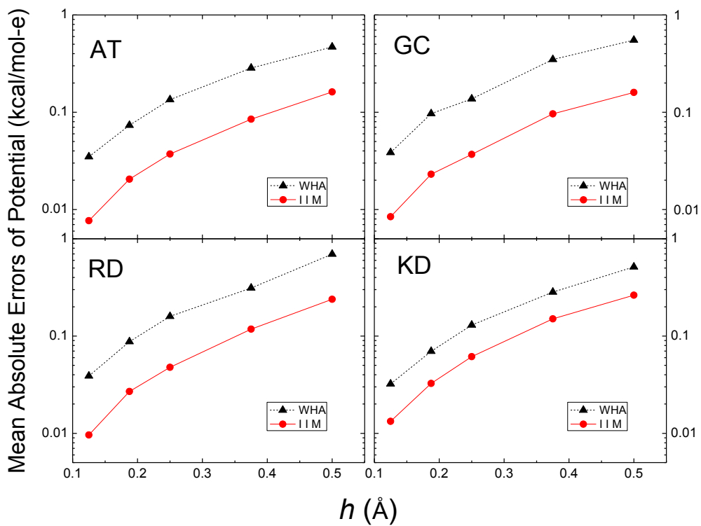
Figure 5. Mean absolute errors of reaction field potentials at the irregular grid points (inside, kcal/mol-e) versus grid spacing h (Å) with respect to those calculated at the fine grid spacing of 1/16\text{Å} for AT, GC, RD and KD dimers, respectively.
