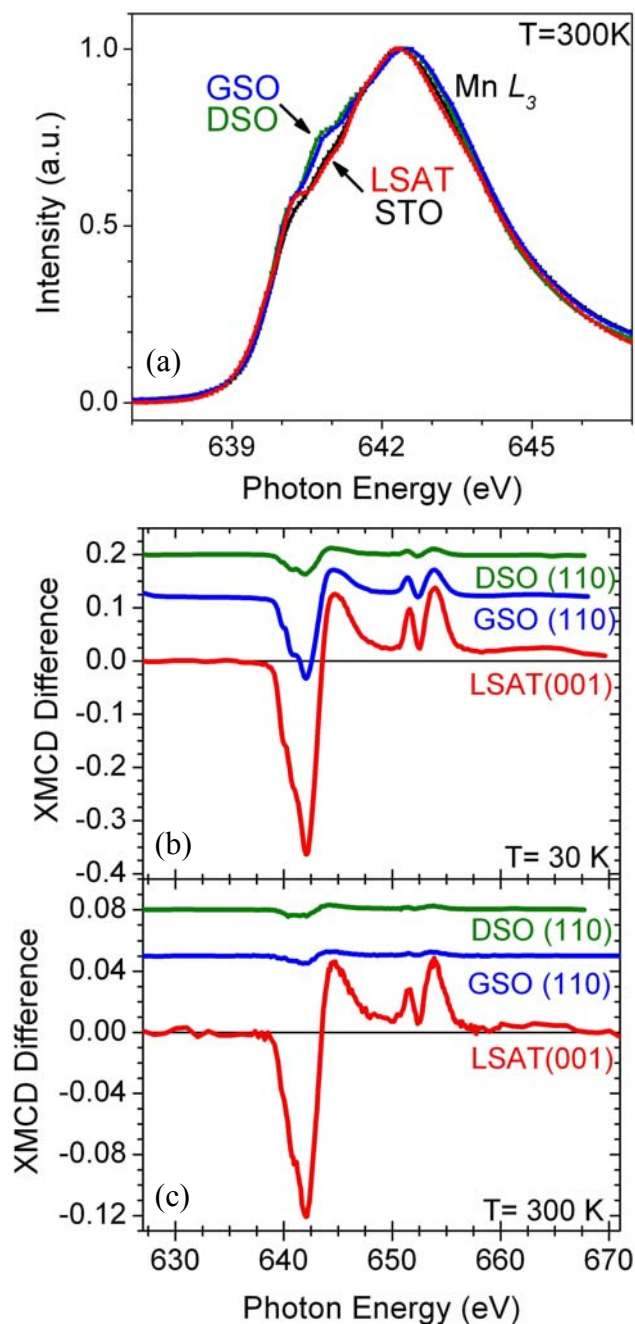
Figure 1: (a) XA spectra of the \text{Mn } L_3 edge and XMCD difference spectra measured at (b) 30 K and (c) 300 K for a 35 nm thick LSMO films on LSAT, GSO, and DSO substrates.
