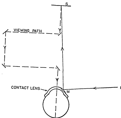
FIG. 2. Diagram of an apparatus used to produce a retinal image which remains stationary on the retina in spite of eye movements. Rays from projector P are reflected from mirror M , mounted on the contact lens. The rays form an image of a fixation target at screen S . The subject views the target through the dashed viewing path. When the eye moves through angle \alpha , the projected image moves through 2\alpha . Since the length of the viewing path is twice the distance from M to S , the retinal image enters the eye at angle \alpha . Therefore the retinal image does not move with respect to the retina. (After Riggs, Ratliff, Cornsweet, and Cornsweet. 4 )
