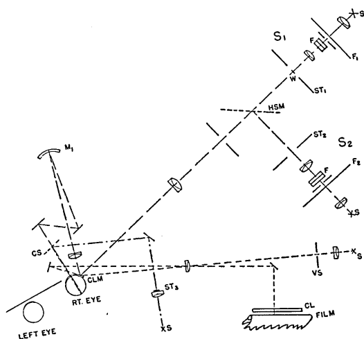
FIG. 3. Diagram of the present optical apparatus. S_1 and S_2 two projection systems; S 's ribbon filament sources; F_1 and F_2 synchronized flicker vanes; F 's filter holders; ST_1 and ST_2 stops with circular apertures; W the stimulus wire; HSM a half-silvered mirror; CLM mirror mounted on the contact lens; M_1 a Mangin mirror; ST_3 a circular stop; CS a microscope cover slip; VS a vertical slit opening; CL a horizontal cylindrical lens.
