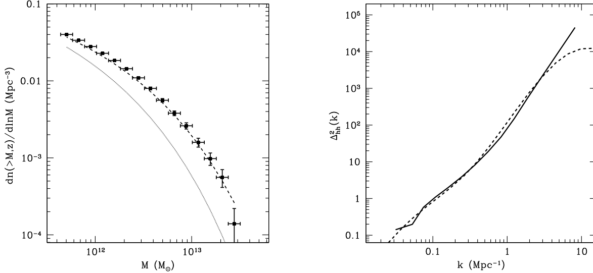
Figure 1. Left panel: The calculated halo mass function shown as points. The dotted curve is the Press-Schechter analytic mass function. The dashed curve shows the Sheth-Tormen mass function, which agrees with our results by construction. Right panel: Halo power spectra. The solid line represents the halo power spectrum measured from our standard ( L = 250 Mpc) box, and the dashed line is the halo model analytic equivalent.
