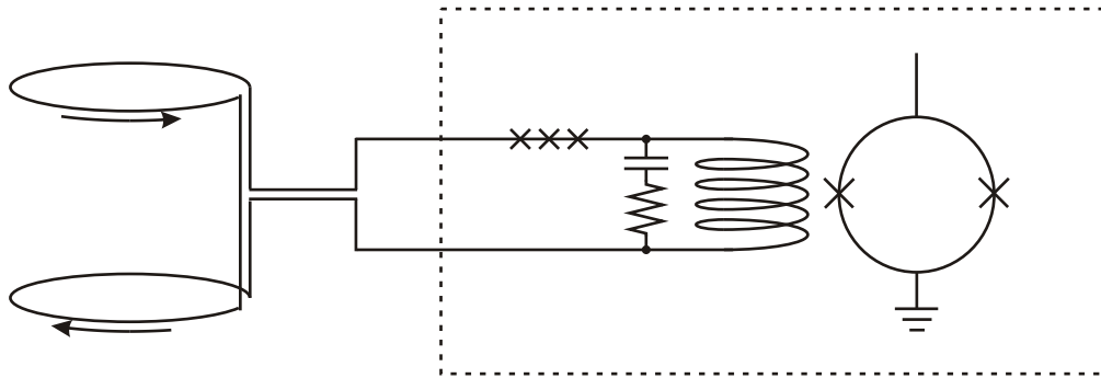
Fig. 2.6: Flux transformer with Josephson junction array in series with input coil. For simplicity, only three junctions are shown.
