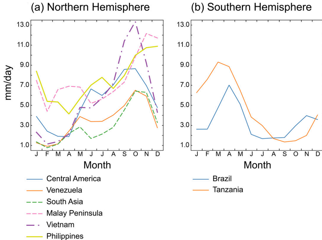
FIG. 2. The climatological annual cycle of precipitation ( \text{mm day}^{-1} ) averaged over the areas that receive more than half of their annual rainfall in local autumn and winter in (a) the Northern Hemisphere and (b) the Southern Hemisphere. Spatial averaging was performed over the land areas within the boxes indicated in Fig. 1 using CHIRPS data with locations receiving less than half of their annual rainfall in autumn and winter excluded.
