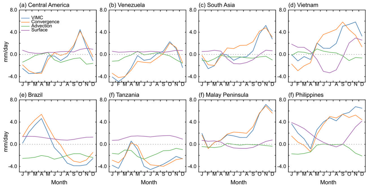
FIG. 10. The climatological annual cycle of the advection, convergence, and surface terms calculated in the budget of moisture convergence using ERA5 monthly means for each of the autumn monsoon regions.
