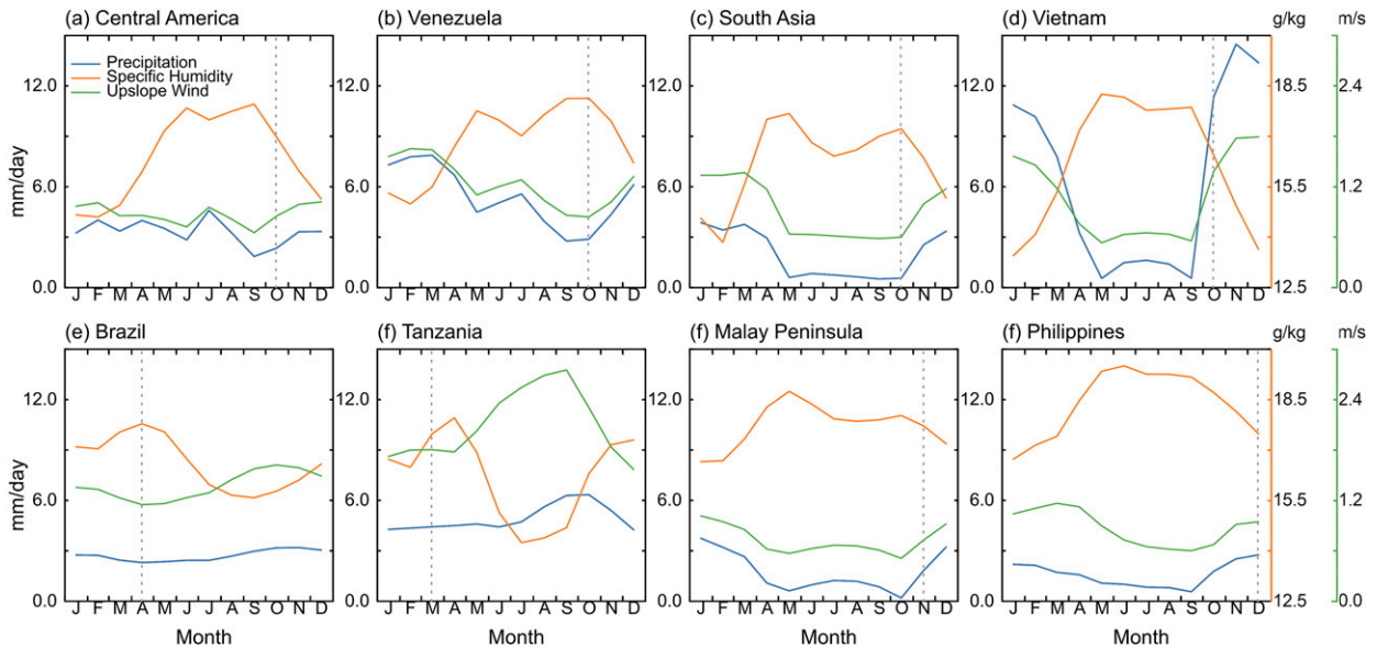
FIG. 8. The seasonal cycle of precipitation over autumn monsoon regions predicted by the model of stable upslope ascent, with the surface specific humidity and wind speed in the direction normal to the slope of the surface that were used as inputs. The y axes for specific humidity (orange; \text{g kg}^{-1} ) and wind speed (green; \text{m s}^{-1} ) are shown on the right. Regions with downslope winds and therefore negative predicted precipitation were set to zero before spatial averaging, and ocean regions were excluded. The dotted lines indicate the month of maximum climatological precipitation in each region from Fig. 2.
