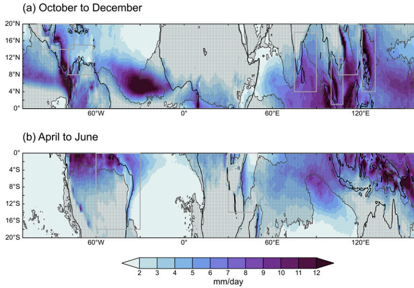
FIG. 3. The climatological precipitation ( \text{mm day}^{-1} ) averaged over late autumn and early winter in the (a) Northern and (b) Southern Hemisphere [October–December in (a) and April–June in (b)] from TRMM. The gray contour demarcates areas that receive more than half of their annual rainfall in local autumn and winter [September–February in (a) and March–August in (b)]; regions that receive more than half of their annual rainfall during spring and summer are stippled. Light gray boxes indicate the regions used for averaging in sections 6 and 7.
