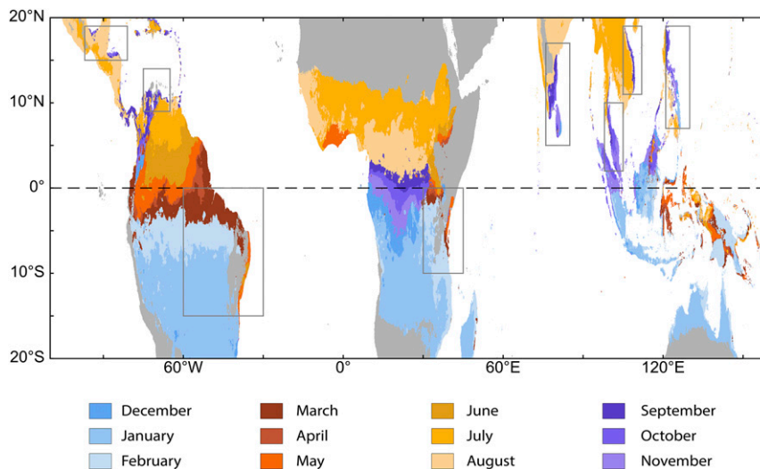
FIG. 4. The climatological month of maximum precipitation at each location from CHIRPS, after a 5-month running mean was applied to the annual cycle. Regions with annual-mean rainfall less than 2 \text{ mm day}^{-1} are indicated in gray.
