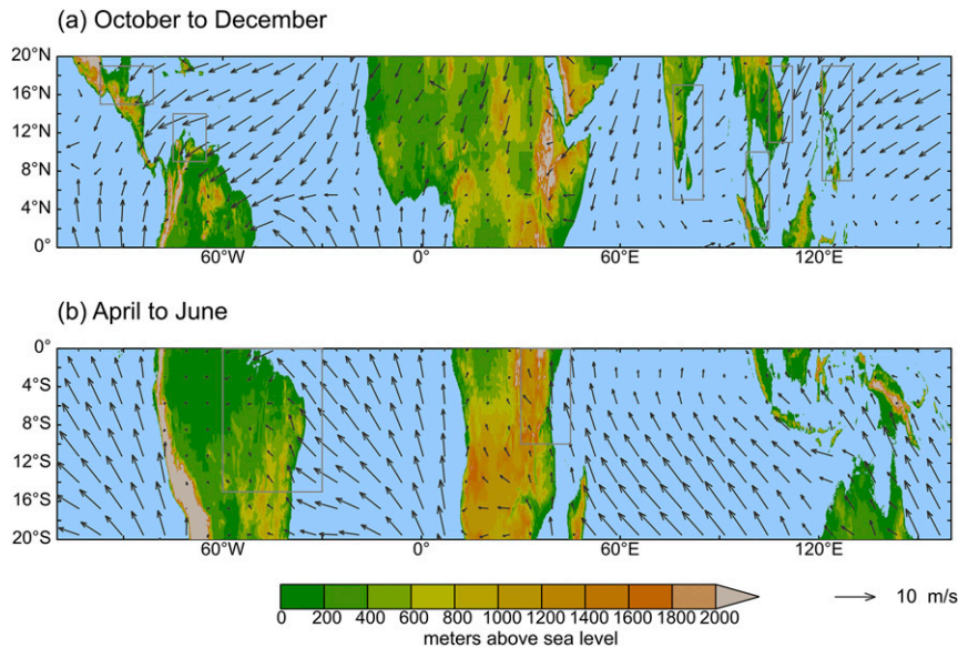
FIG. 6. The height of the land surface above sea level (colors) and the climatological seasonal-mean wind field at 10 m above the surface (arrows) in (a) October–December in the Northern Hemisphere and (b) April–June in the Southern Hemisphere.
