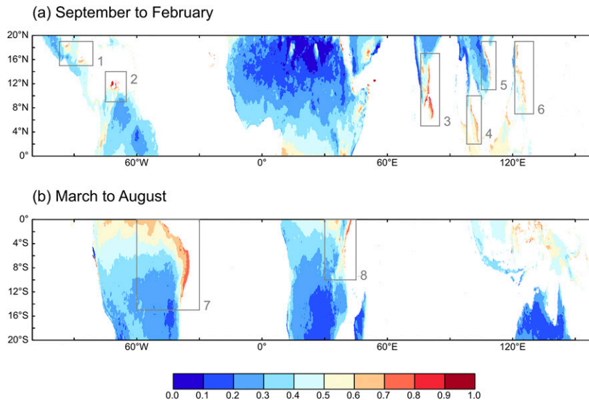
FIG. 1. The climatological fraction of annual rainfall that occurs during the fall and winter months in (a) the Northern Hemisphere (September–February) and (b) the Southern Hemisphere (March–August). Shades of red and orange indicate regions where half or more of the annual rainfall occurs during these months. Gray boxes highlight the eight regions examined in this study, numbered as in the text of section 3.
