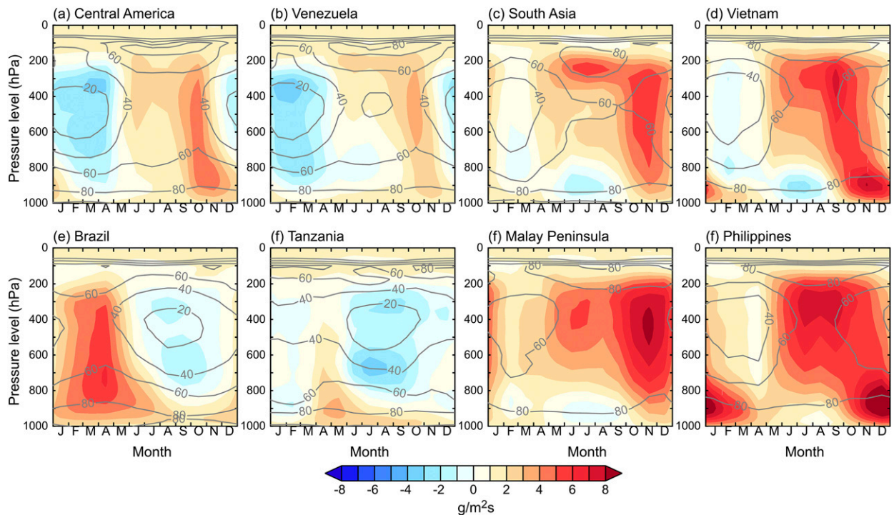
FIG. 11. The climatological annual cycles of vertical mass flux (colors) and relative humidity as a percentage (contours) averaged over each of the autumn monsoon regions.
