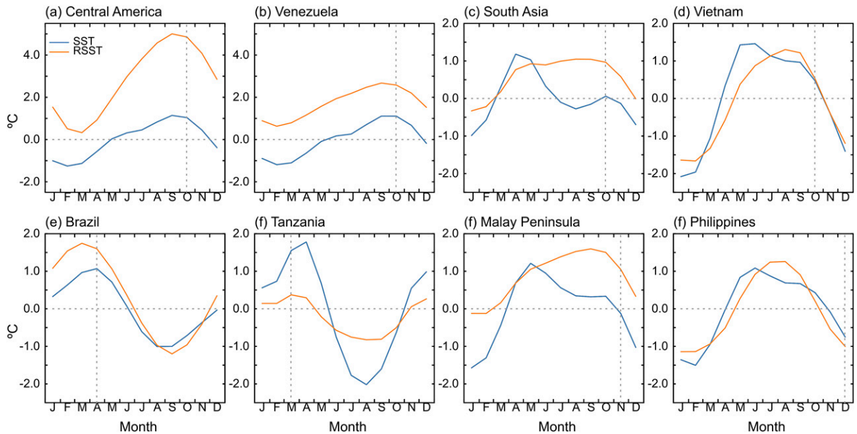
FIG. 12. The climatological annual cycles of SST and RSST in each of the autumn monsoon regions. The annual-mean SST was subtracted from the climatological values of SST for each region. (a),(b) Note the different y axis range, which is due to the high values of RSST in their annual cycle. The vertical dotted line indicates the month of maximum precipitation over land from Fig. 2.
