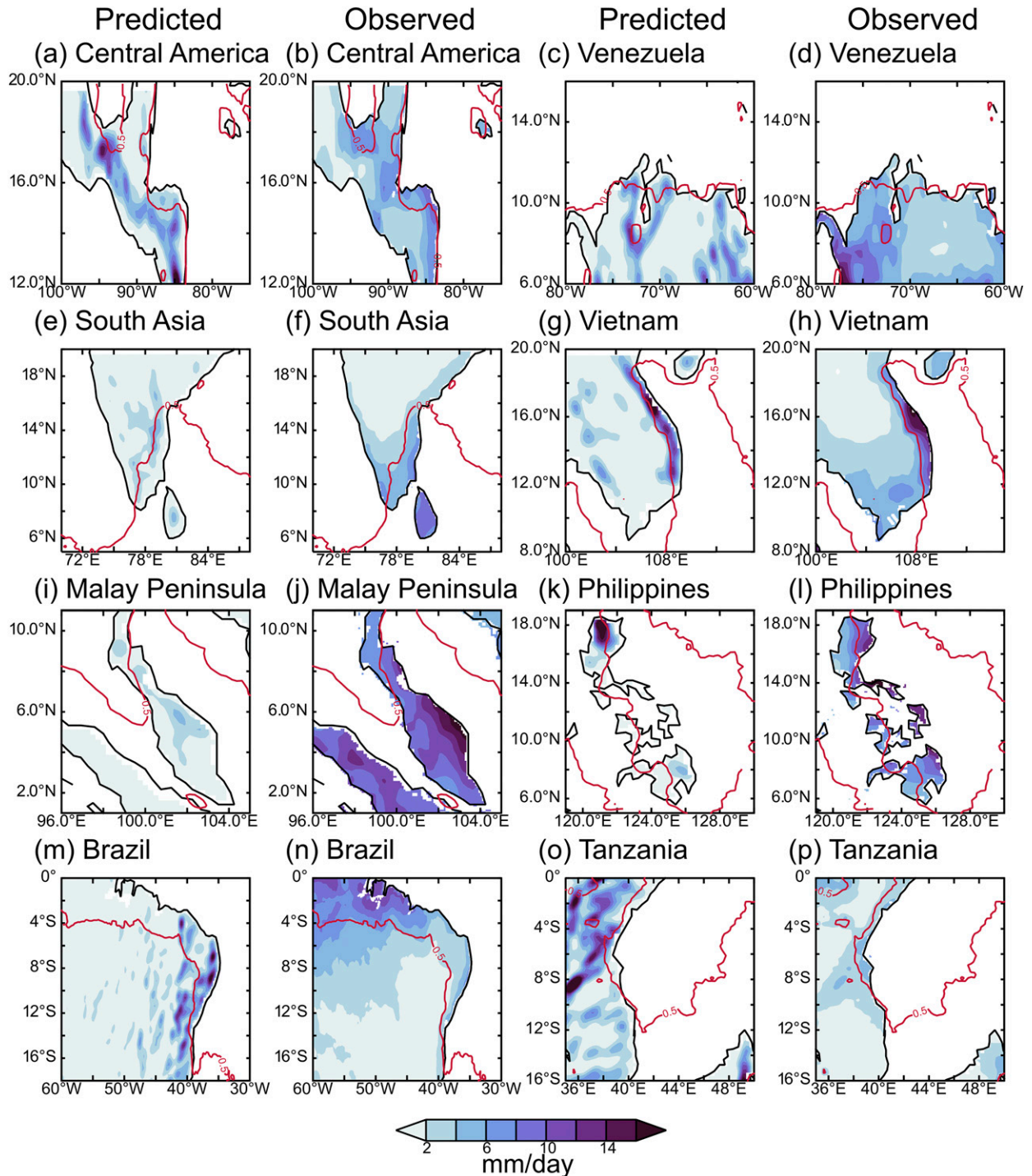
FIG. 7. The climatological precipitation (first and third columns) predicted by the orographic model and (second and fourth columns) from TRMM for comparison in each region, averaged over (a)–(l) October–December in the Northern Hemisphere and (m)–(p) April–June in the Southern Hemisphere. The red contour demarcates the regions that receive more than half of their annual rainfall in autumn and winter.
