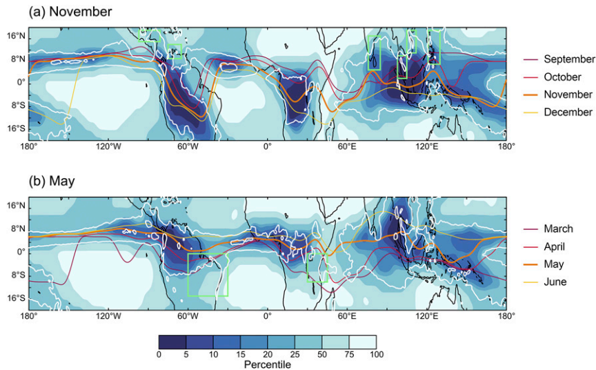
FIG. 5. The percentile of outgoing longwave radiation (OLR) with respect to the climatological distribution of OLR over the tropics in (a) November and (b) May (colors). An uneven color scale is used to highlight the lower percentiles, which suggest convective activity. Contours of 5 and 15 mm day -1 of climatological precipitation are shown for the corresponding months in white contours. Colored lines in (a) and (b) indicate the latitude of minimum OLR within the tropics during boreal and austral autumn, respectively (see legend), with bold orange lines representing the month for which the other variables in each panel are shown. The latitude of minimum OLR has been smoothed for visualization using a Parzen filter with a window of 7.5°. Green boxes highlight the eight autumn monsoon regions.
