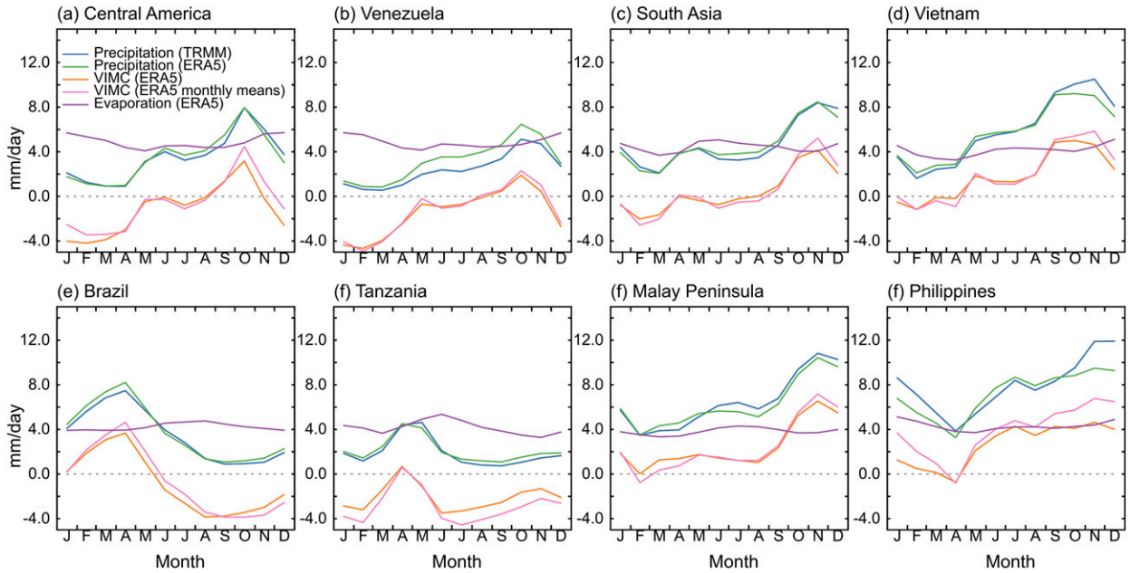
FIG. 9. The monthly climatologies of precipitation, evaporation, and vertically integrated moisture convergence (VIMC) provided in the reanalysis data, and the VIMC calculated from monthly means from ERA5. The climatological precipitation from TRMM averaged over the same regions is included for comparison.
