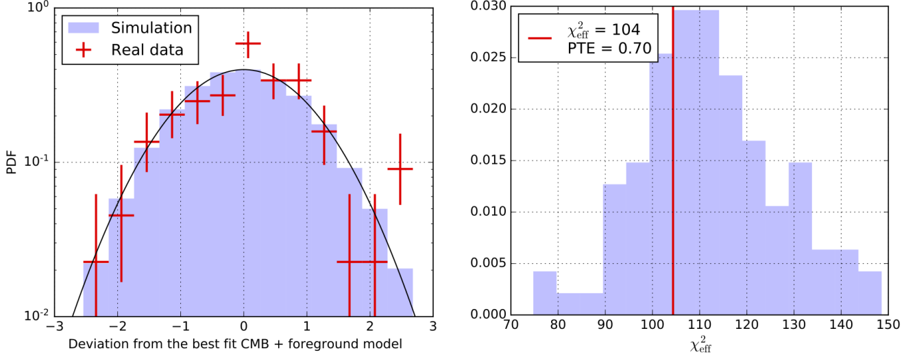
Figure 14. Normalized difference between the measured cross spectra and the best fit CMB+foreground model shown in units of standard deviation (left). Effective \chi^2_{\text{eff}} of the data fit to the model as defined in Equation 27 compared to simulations (right). The distribution shows the 96 simulations and the vertical line indicates the real data.
