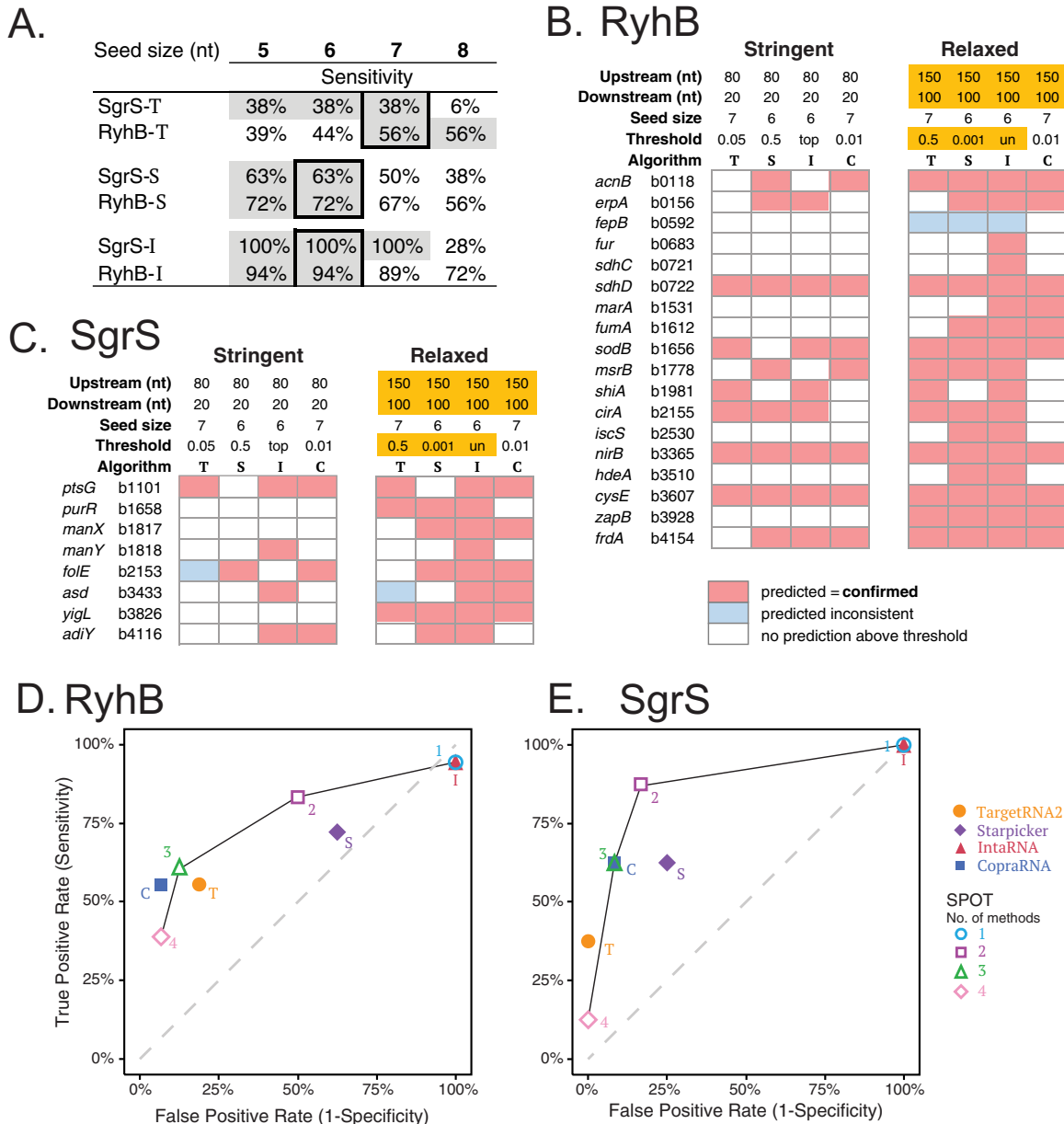
FIG 2 Validation of SPOT using known SgrS and RyhB sRNA-mRNA interactions. (A) Seed size indicates the number of consecutive base pairing nucleotides in an sRNA-mRNA interaction prediction. This is an adjustable parameter for each algorithm. Seed sizes were varied from 5 to 8 nt, and the sensitivity (true positive rate) was determined for known SgrS and RyhB interactions, while all other parameters were kept constant. Optimal seed sizes (shown in boxes outlined by thick black lines) were chosen for each algorithm. The highest percentage values for sensitivity are indicated with gray shading. Algorithms were abbreviated and are indicated after the sRNA or mRNA as follows: -T for TargetRNA2, -S for sTarPicker, and -I for IntaRNA. (B and C) Analyses were rerun using optimal seed sizes identified in panel A, but using a stringent parameter set with a narrow window size and high individual significance thresholds or a relaxed parameter set with a wider window size and low individual significance thresholds. Correctly predicted interactions for RyhB and SgrS are shown as pink cells, predictions that were inconsistent with confirmed interaction sites are shown in blue, and empty cells did not have any predictions above the indicated thresholds. Algorithms are abbreviated as follows: T for TargetRNA2, S for sTarPicker, I for IntaRNA, and C for CopraRNA. (D and E) RyhB and SgrS have experimentally validated (true-positive) and invalidated (true-negative) mRNA targets, which were used to generate receiver operating characteristic (ROC) curves. These plots enable assessment of the accuracy of SPOT and the individual algorithms. Using the relaxed search parameters, two-algorithm agreement in SPOT had greater true-positive rates and more acceptable false-positive rates compared with individual algorithms with the same settings.
