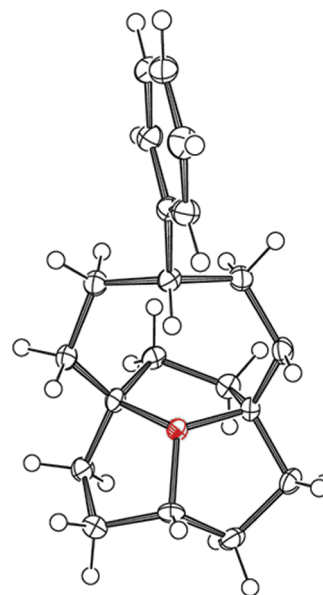
Figure 3. X-ray crystal structure of the \text{C}_6\text{H}_6 addition product to cation 8 . The counterion is omitted for clarity.
