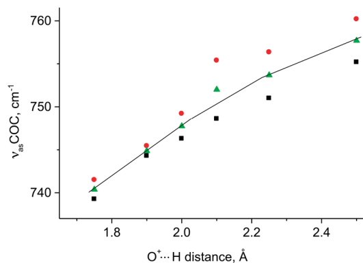
Figure 1. Dependence of \nu_{\text{asCOC}} stretches (red, black; average green) on O...H distance in calculated 2...HCl pairs.
