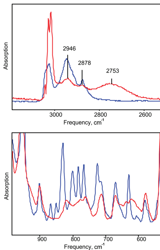
Figure 2. IR spectra (normalized to unit intensity of the carborane anion) of alkene 7 before (blue) and after (red) grinding with \text{H}\{\text{Cl}_{11}\} .
