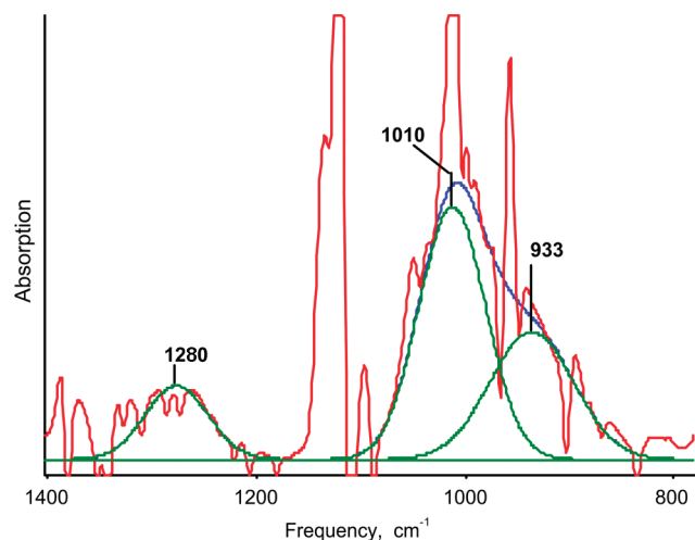
Figure 6. Deconvolution (green), with summation (blue), of IR spectrum of 6b[\text{H}\{\text{Cl}_{11}\}_2] with the spectrum of \{\text{Cl}_{11}\} anion subtracted (red).
