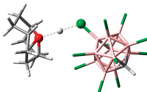
Figure 5. Graphical depiction of the experimental results described in section 4.4.
