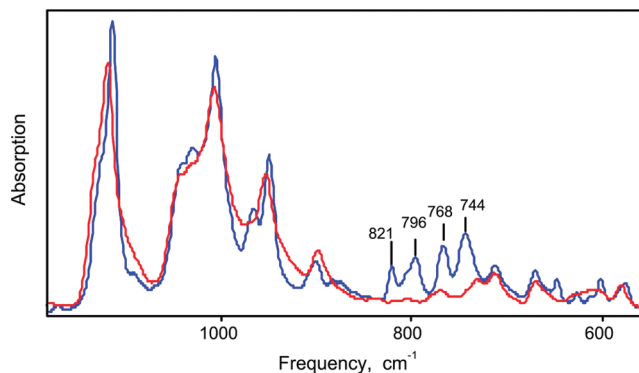
Figure 7. IR spectrum of the product from 1:2 mol ratio of 6a\{\text{Cl}_{11}\} and \text{H}\{\text{Cl}_{11}\} in liquid HCl (red) compared to 6a\{\text{Cl}_{11}\} (blue).
