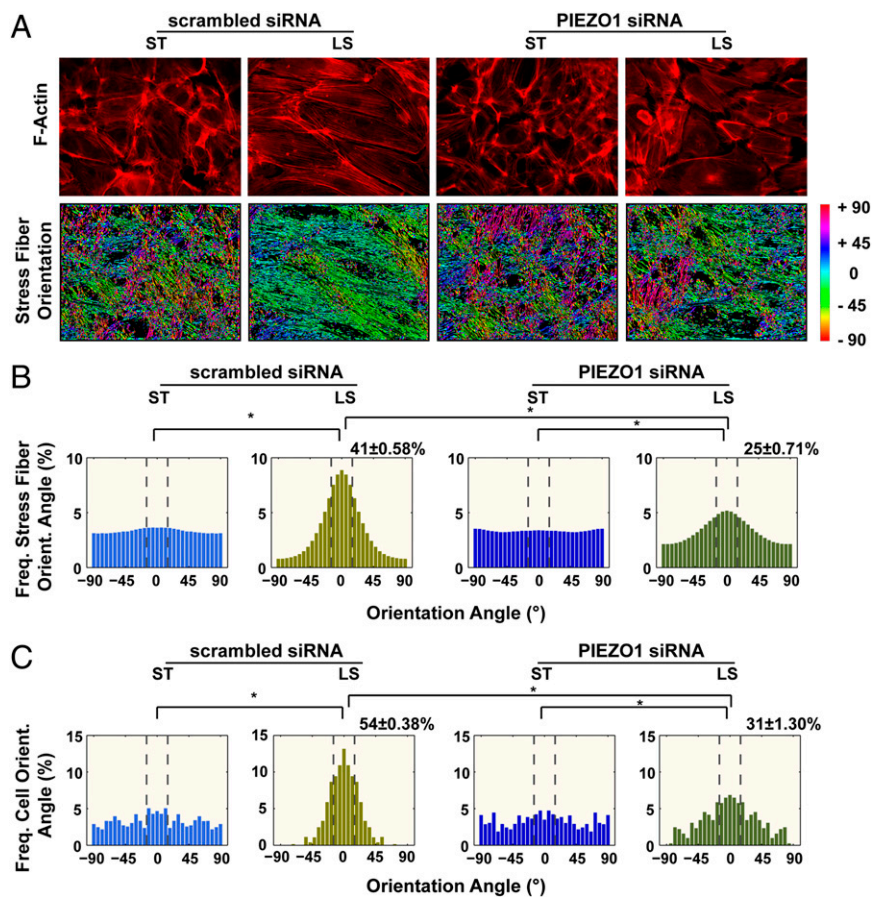
Fig. 5. Knockdown of PIEZO1 leads to defects in cellular alignment upon laminar shear stress. (A) F-actin images stained with TRITC-phalloidin ( Upper ) and angles of stress fiber orientation ( Lower ). Angle measurements were assigned a color code (right) where 0° is parallel to the flow chamber and -90° and 90° are perpendicular. (B) Histograms of stress fiber orientation of cells. (C) Histograms of cell orientation. The mean \pm SEM values refer to percentage of orientations between \pm 15^\circ for three independent biological experiments. Total numbers of cells analyzed are 348 (ST) and 236 (LS) for scrambled siRNA and 290 (ST) and 170 (LS) for PIEZO1 siRNA. ST, static; LS, laminar shear for 24 h. Asterisk indicates significant difference by Watson's U2 test.
