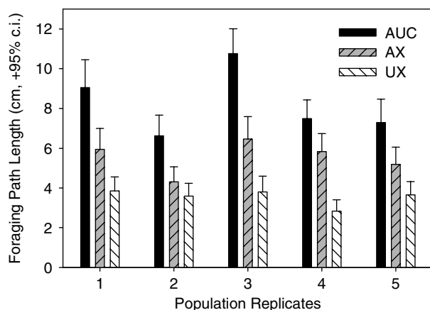
Fig. 2. The foraging path length of the ammonia-resistant populations (AX), urea-resistant populations (UX), and their controls (AUC).
