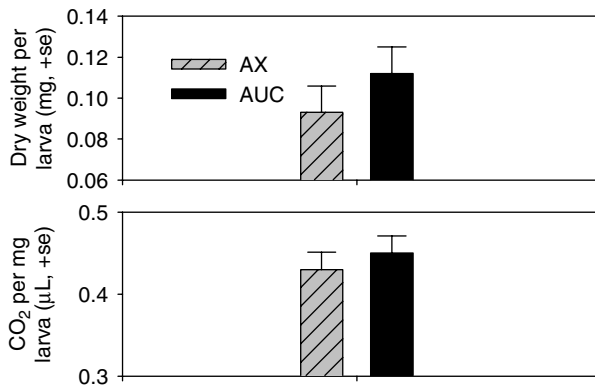
Fig. 3. Average physiological measurements on 72-h larvae in the ammonia-resistant populations (AX) and their controls (AUC). The top panel shows the average dry weight per larva, and the bottom panel shows the amount of CO 2 produced per mg of larva.
