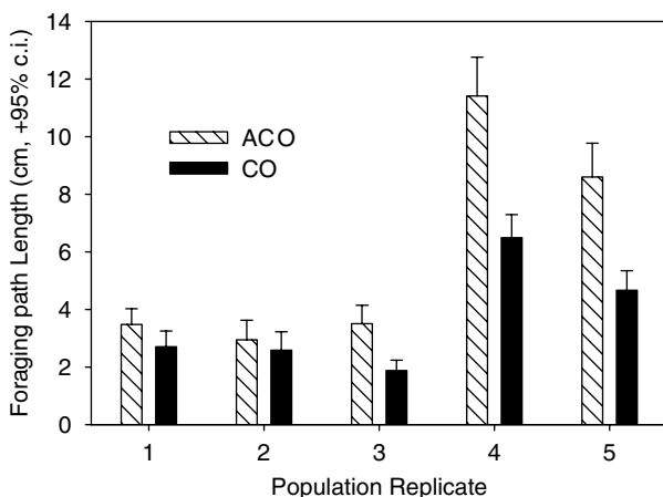
Fig. 1. The foraging path length in the five accelerated development populations (ACO) and their controls (CO).
