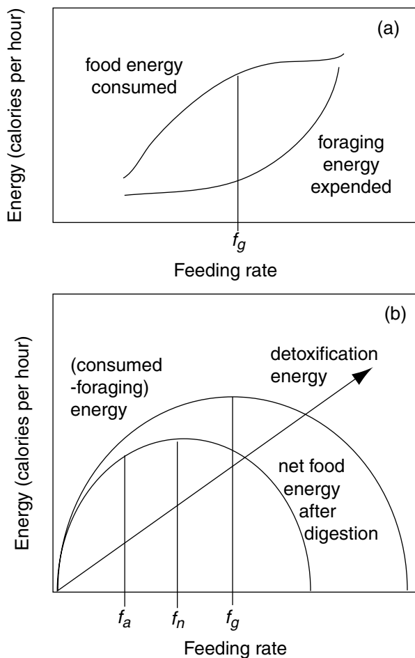
Fig. 4. The relationship between larval feeding rates and energy acquisition. As feeding rates increase, there will be a general increase in the amount of food consumed, although gain is expected to slow at high feeding rates (a). High feeding rates also expend more energy resulting in a feeding rate, f_g , which maximizes the gross amount of energy intake (a). (b) The difference between the food energy consumed and the energy used for foraging is shown as a function of feeding rates. Below that curve is a second curve showing the net energy available to the larva after digestion (see text for additional discussion). Environments with high levels of ammonia require energy to detoxify the ingested ammonia. This energy is shown as a straight line. The difference between the net energy curve and the detoxification line represents energy available after detoxification, which is maximized at f_a .
