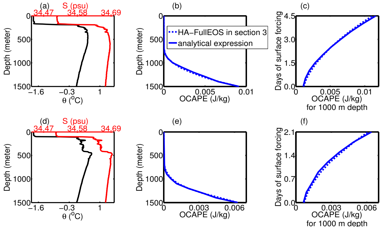
FIG. 4. (a) Profiles of potential temperature ( \theta ) and salinity ( S ) from the wintertime Weddell Sea, obtained from Maud Rise ( 65.4605^{\circ}\text{S} , 2.4007^{\circ}\text{E} ) on August 2, 1994, ANZFLUX CTD profile station 48 (courtesy of Bruce Huber; McPhee et al. 1996). (b) OCAPE vs the depth of the profiles shown in panel (a); at each depth we computed the OCAPE, assuming that depth to be the bottom of the ocean (i.e. not permitting any adiabatic rearrangement of the fluid below that depth). The dashed and solid blue lines are from the HA-FulleOS in section 3 and the analytical solution derived from section 4d, respectively (see section 5 for details). (c) Estimated temporal evolution of OCAPE for 1000 m depth of profiles in panel (a) during a winter surface brine rejection forcing. This forcing equals an ice formation rate of 1.5 cm/day, which is common for the winter Weddell Sea (Harcourt 2005; Lange et al. 1989). Calculation methods are described in the text of section 5. (d,e,f) As (a,b,c) but for profiles observed over Maud Rise ( 65.5177^{\circ}\text{S} , 1.1315^{\circ}\text{E} ) on August 1, 1994, ANZFLUX CTD profile station 46. 1500 m is approximately the maximum depth of measurement for profiles in both panels (a) and (d). Panels (b), (c), (e) and (f) share the same legend.
