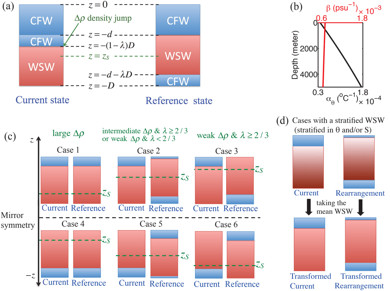
FIG. 2. (a) Schematic of the Current and Reference states for idealized two-layer profiles. The column depth is D , of which \lambda D is WSW and (1-\lambda)D is CFW. There is a downward density jump \Delta\rho \geq 0 at the CFW/WSW interface in the Current state. The densities of adiabatically-repositioned CFW and WSW parcels would be equal at the neutral depth z = z_S . We define d as the thickness of the upper CFW layer in the Reference state. (b) The vertical profile of thermal expansion coefficient \alpha_\theta (black line) and saline contraction coefficient \beta (red line), computed from constant vertical profiles, \theta = -1^\circ\text{C} and S = 34.0 psu, via the full EOS of seawater (Jackett et al. 2006). The linearity of \alpha_\theta and the independence of \beta on depth validate our assumptions in (10a)–(10d). (c) The Current and Reference states of 6 distinct cases, discussed in section 4. The cases are distinguished by the position of the neutral depth z_S (and thus \Delta\rho ) and \lambda , as described in the text. Cases 1–3 have vertical mirror symmetry to Cases 4–6, respectively. (d) Schematic of the “Transformed Current state” and the “Transformed Rearrangement state” discussed in section 4d. Consider a Current state that has a homogeneous CFW overlying a stratified WSW (the stratification is represented by the variation of the red color). We take the mean WSW ( \theta and S ) to define the “Transformed Current state”. Further, we consider a Rearrangement state that is statically-stable (since the Reference state is always statically-stable). Analogously, we take the mean WSW and define a corresponding “Transformed Rearrangement state”.
